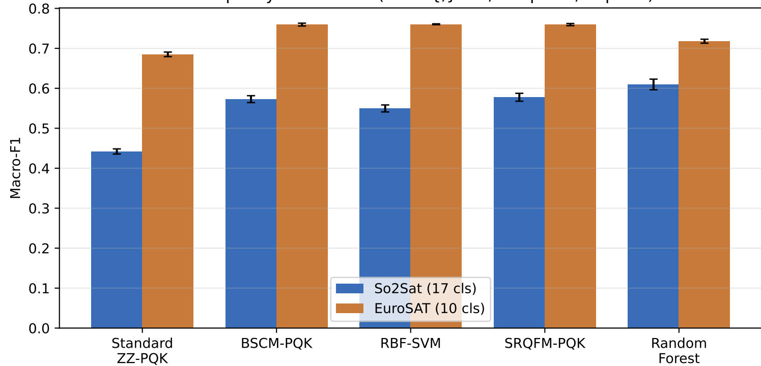
Max-capacity benchmark (N=10{,}000, 16 qubits, depth 6)
