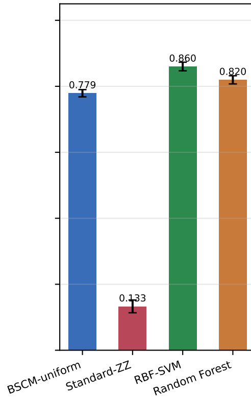
Letter (26 cls, d=16)
