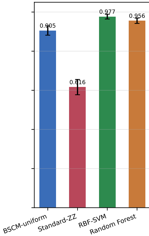
Breast Cancer (2 cls)
