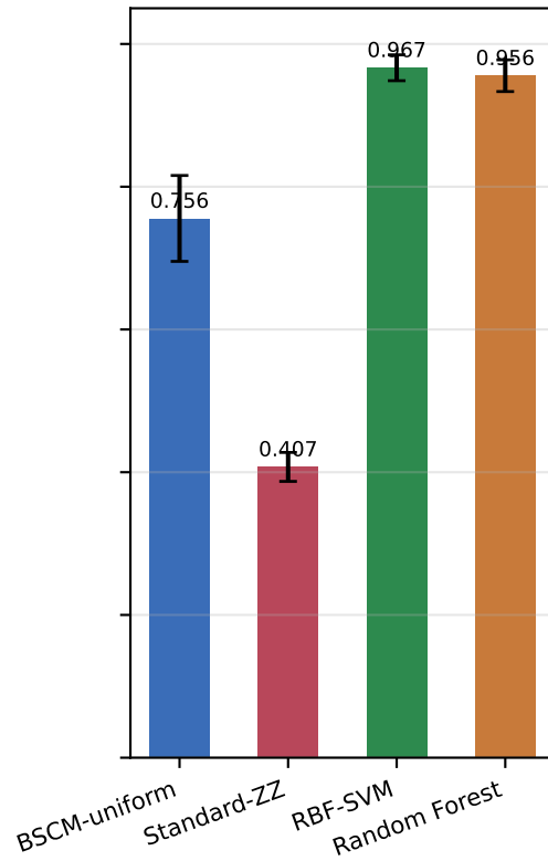
Wine (3 cls, padded)
