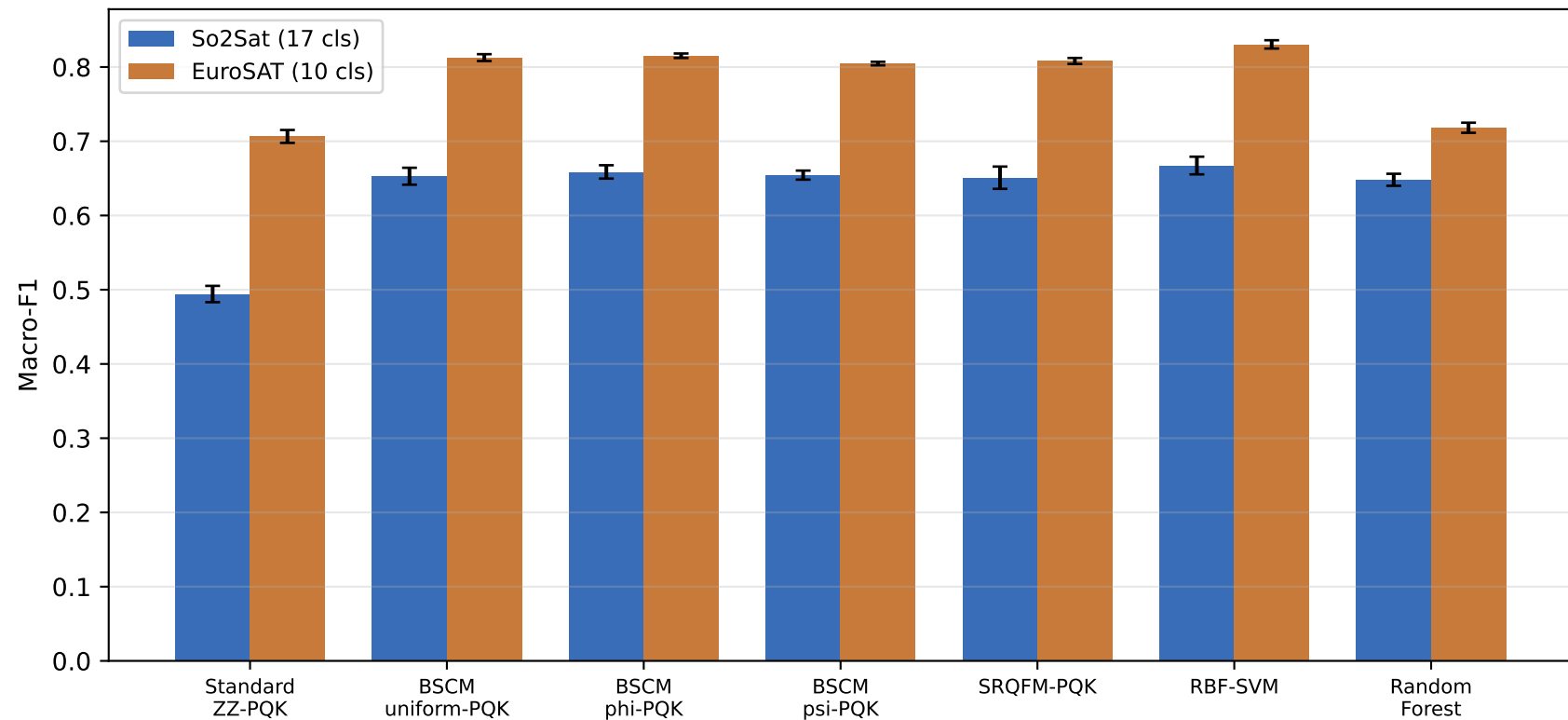
Max-capacity benchmark ( N = 10,000 , 16 qubits, depth L = 6 )
