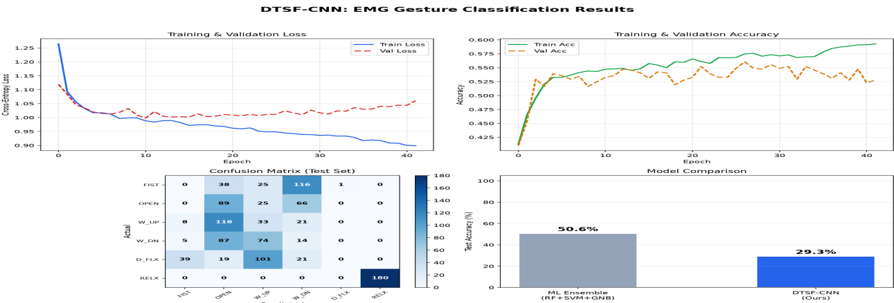
Figure 1: DTSF-CNN Loss / Accuracy Curves & Confusion Matrix
