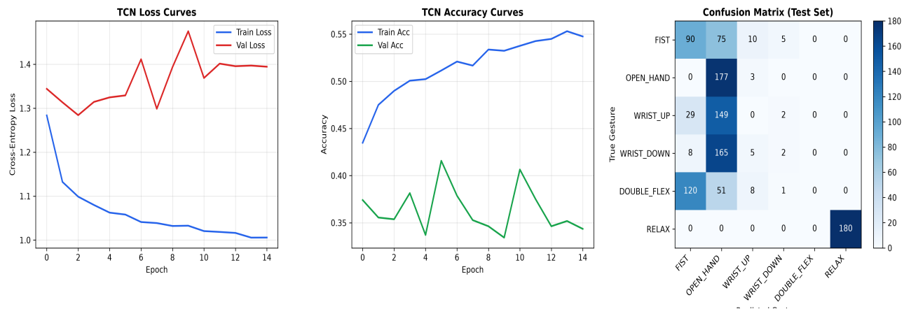
Figure 3: Temporal Convolutional Network (TCN) Evaluation Metrics
