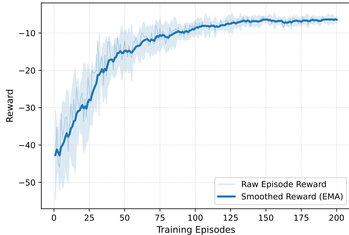
Mean Episode Reward ( R_{\text{striker}} )
