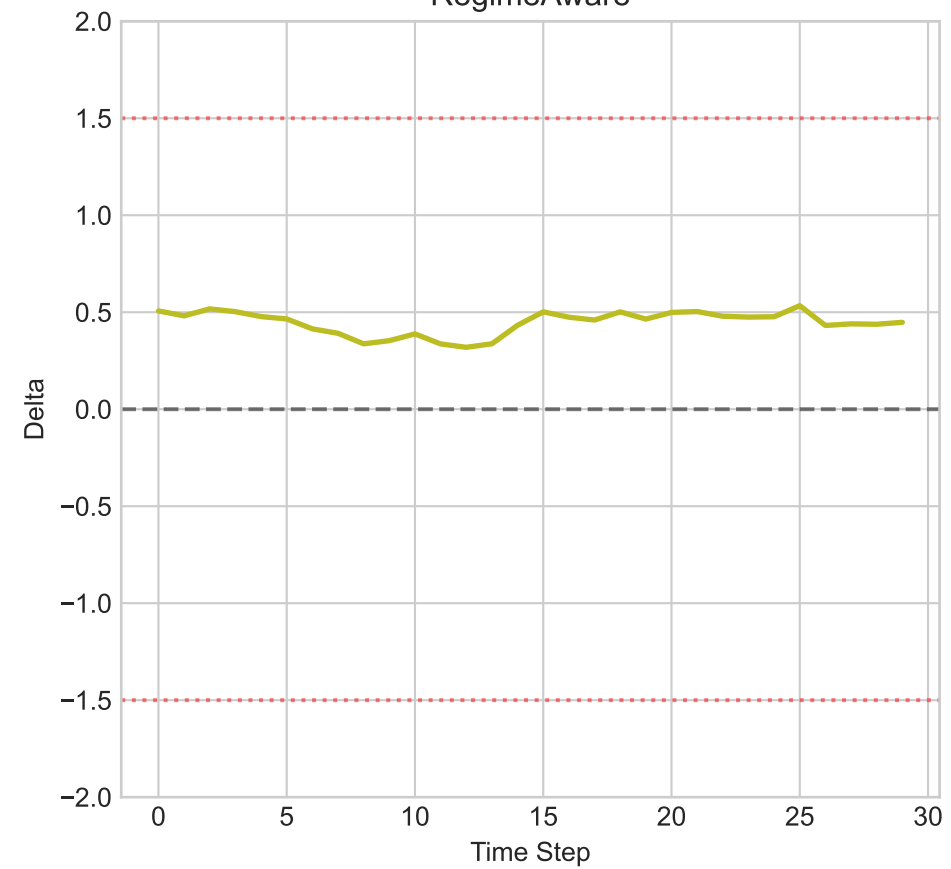
RegimeAware
