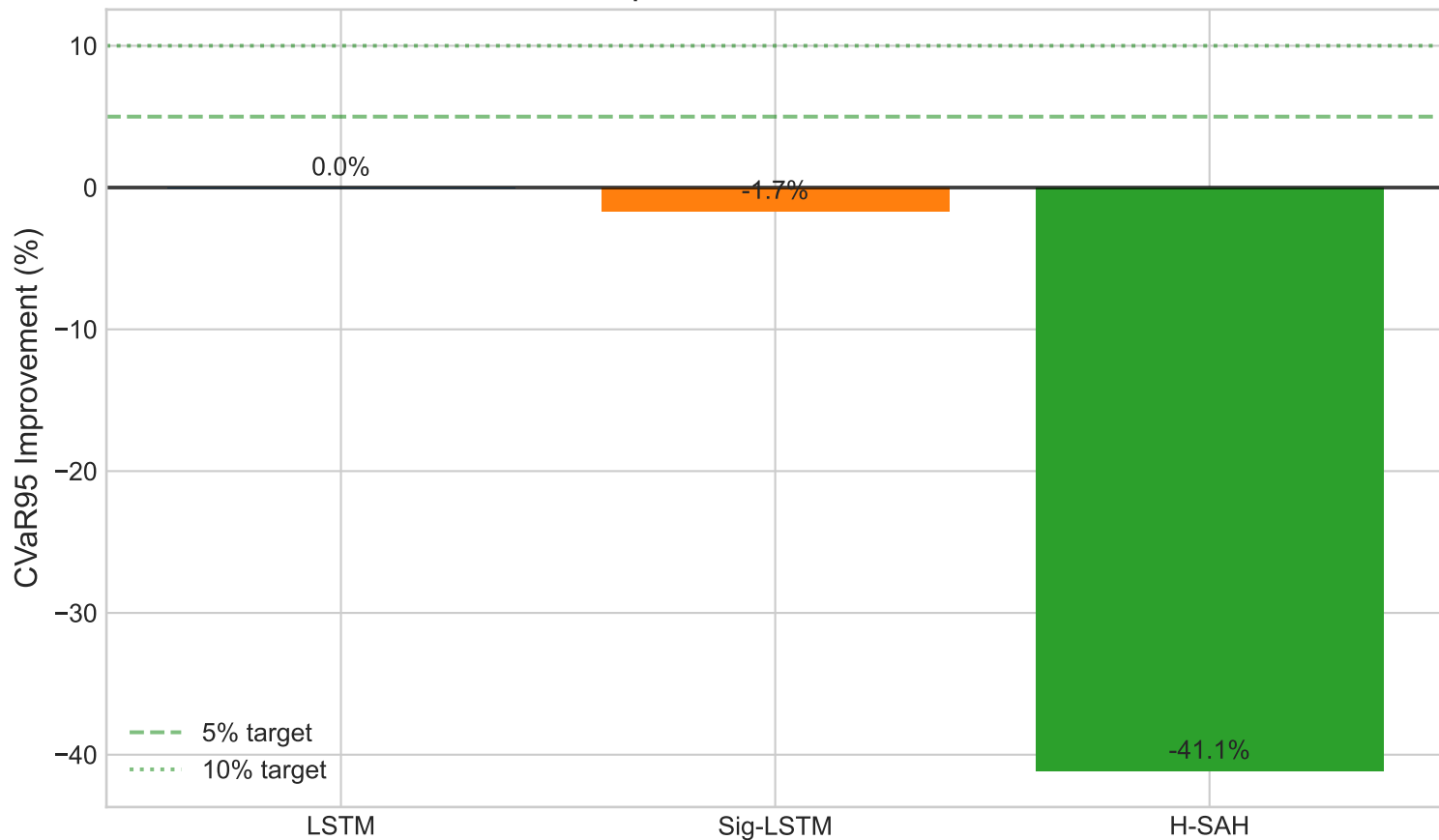
CVaR95 Improvement vs LSTM Baseline
