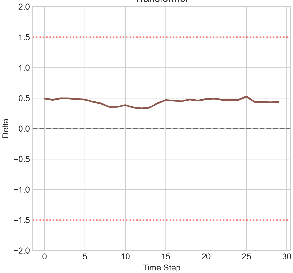
Transformer
