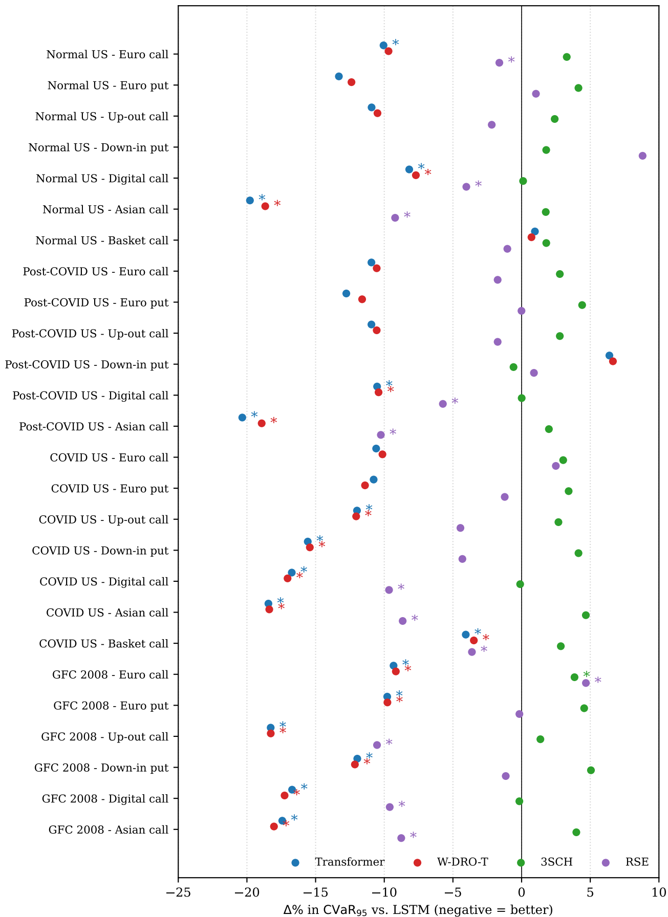
Paired comparison vs. LSTM (* = Holm--Bonferroni significant at \alpha = 0.05 )
