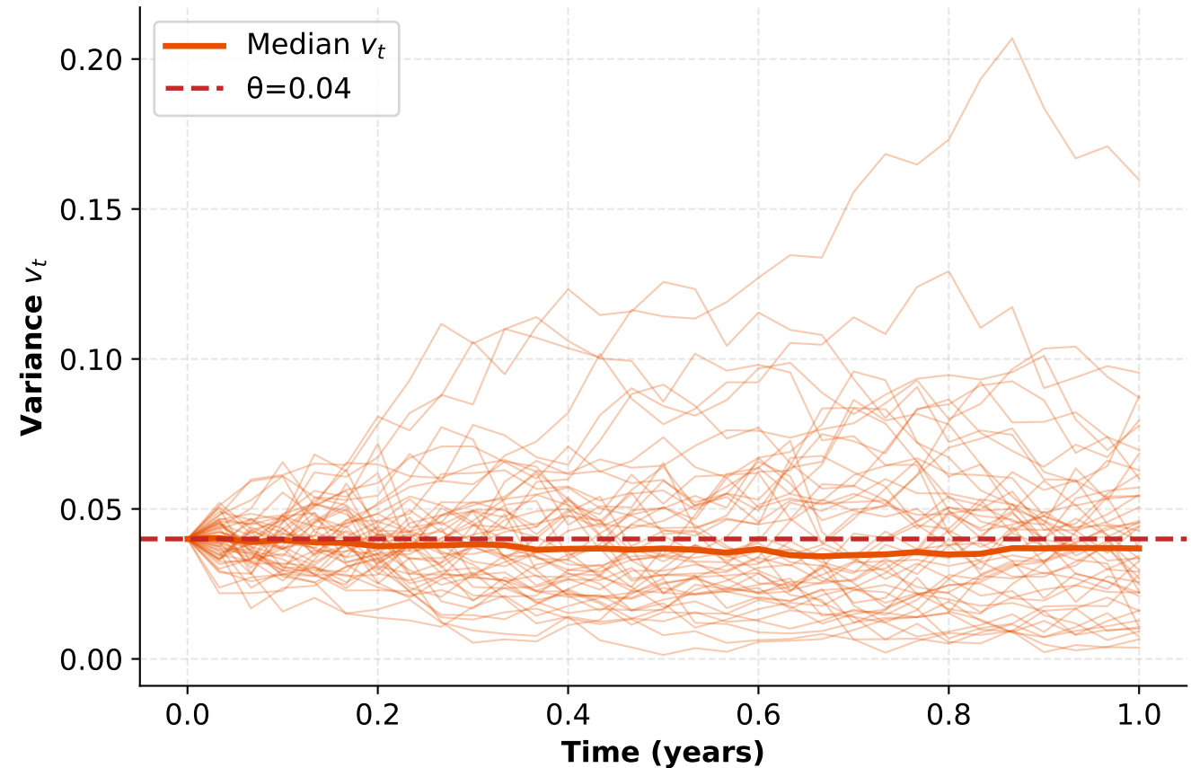
Heston Model — Variance Process
