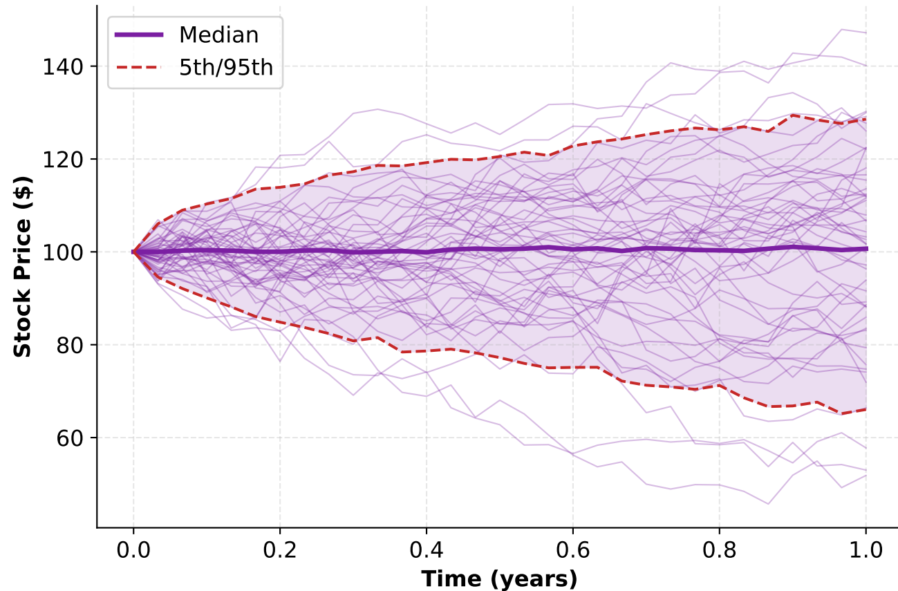
Heston Model — Simulated Stock Paths
