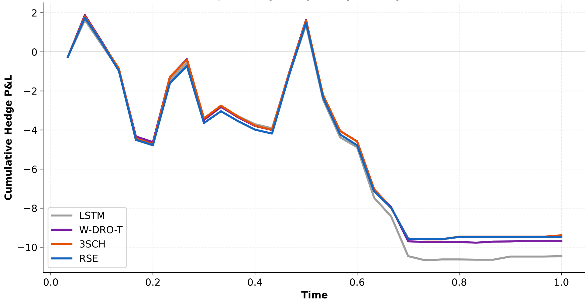
Example Hedge Trajectory — Single Path
