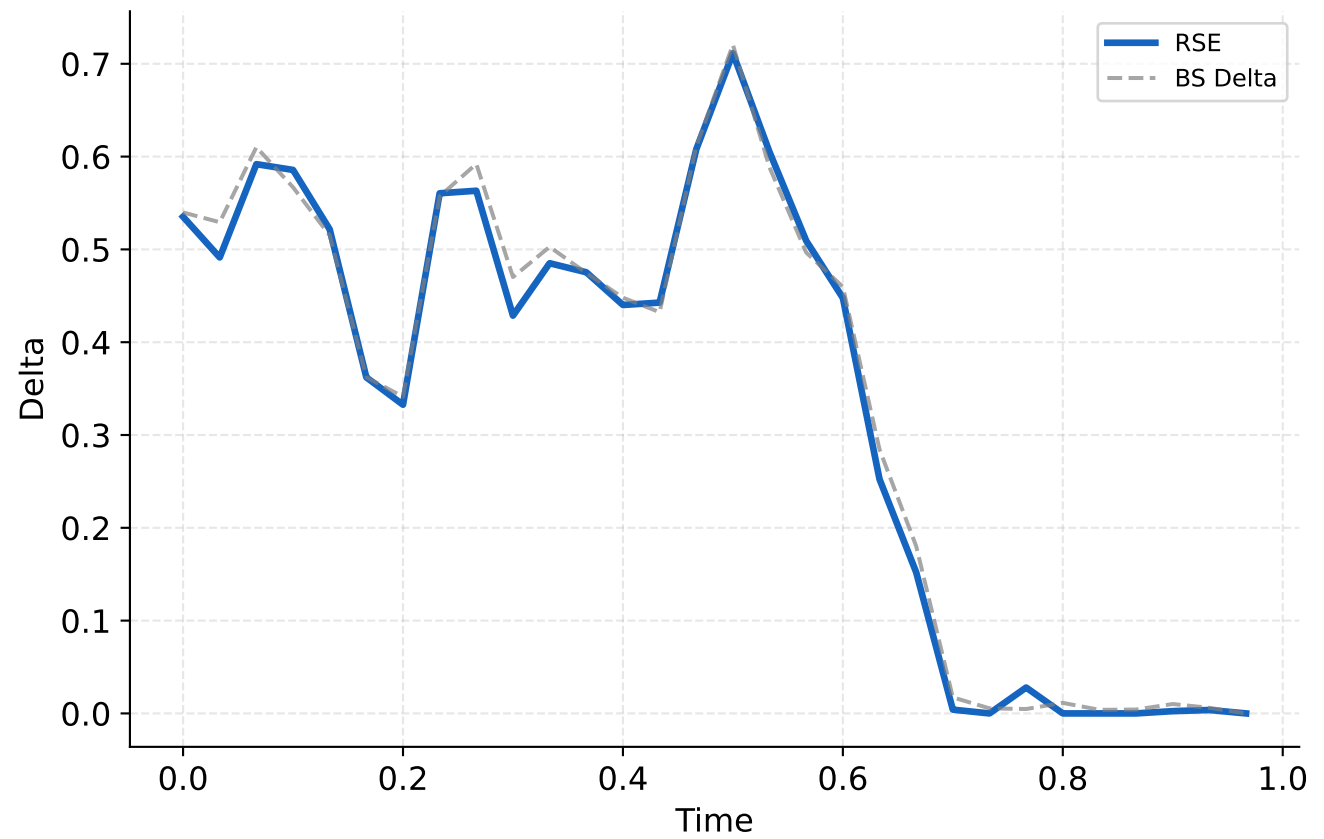
RSE Delta Evolution
