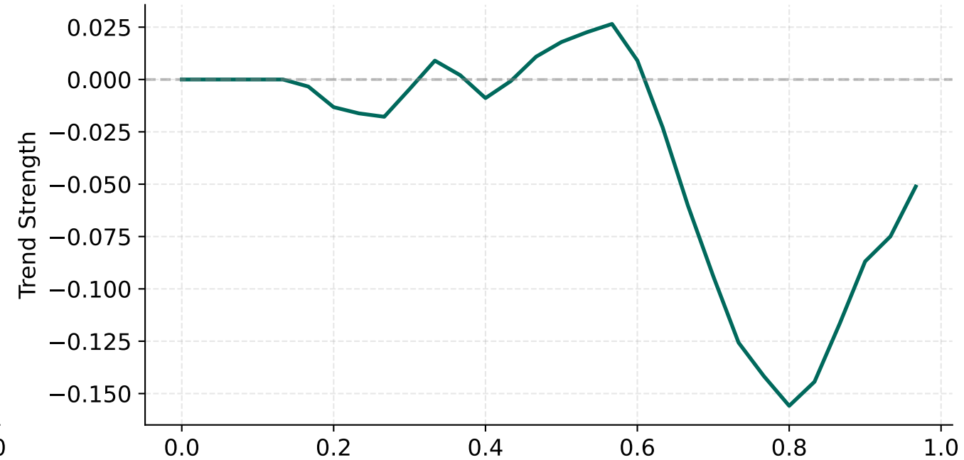
Jump Ratio (RV 2 /BiPV)
