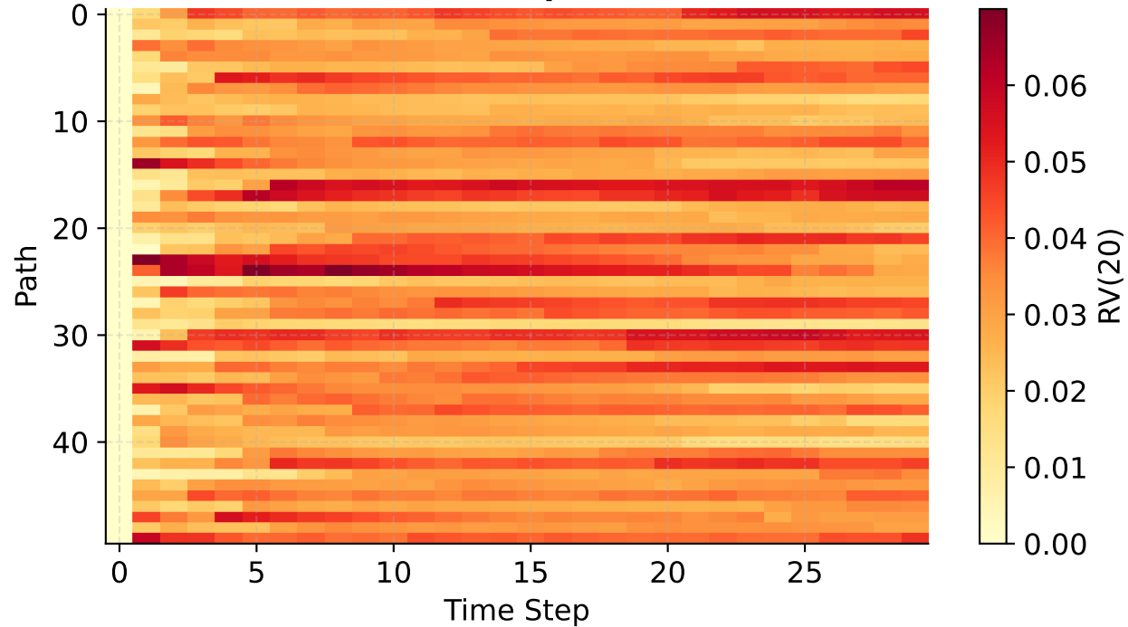
RV(20) Heatmap (50 Paths)
