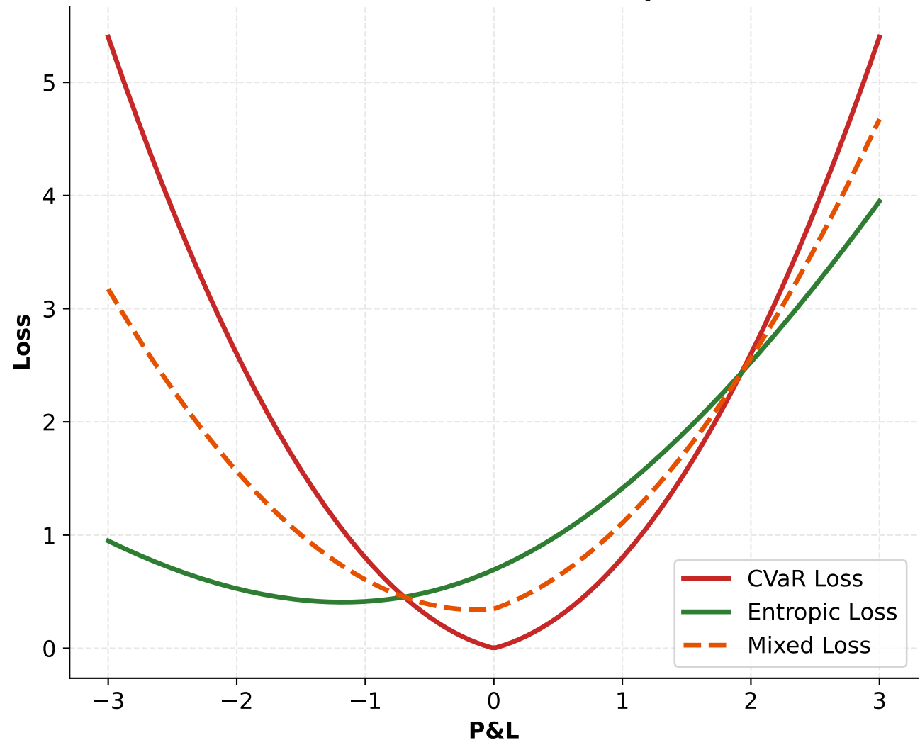
Loss Function Landscape
