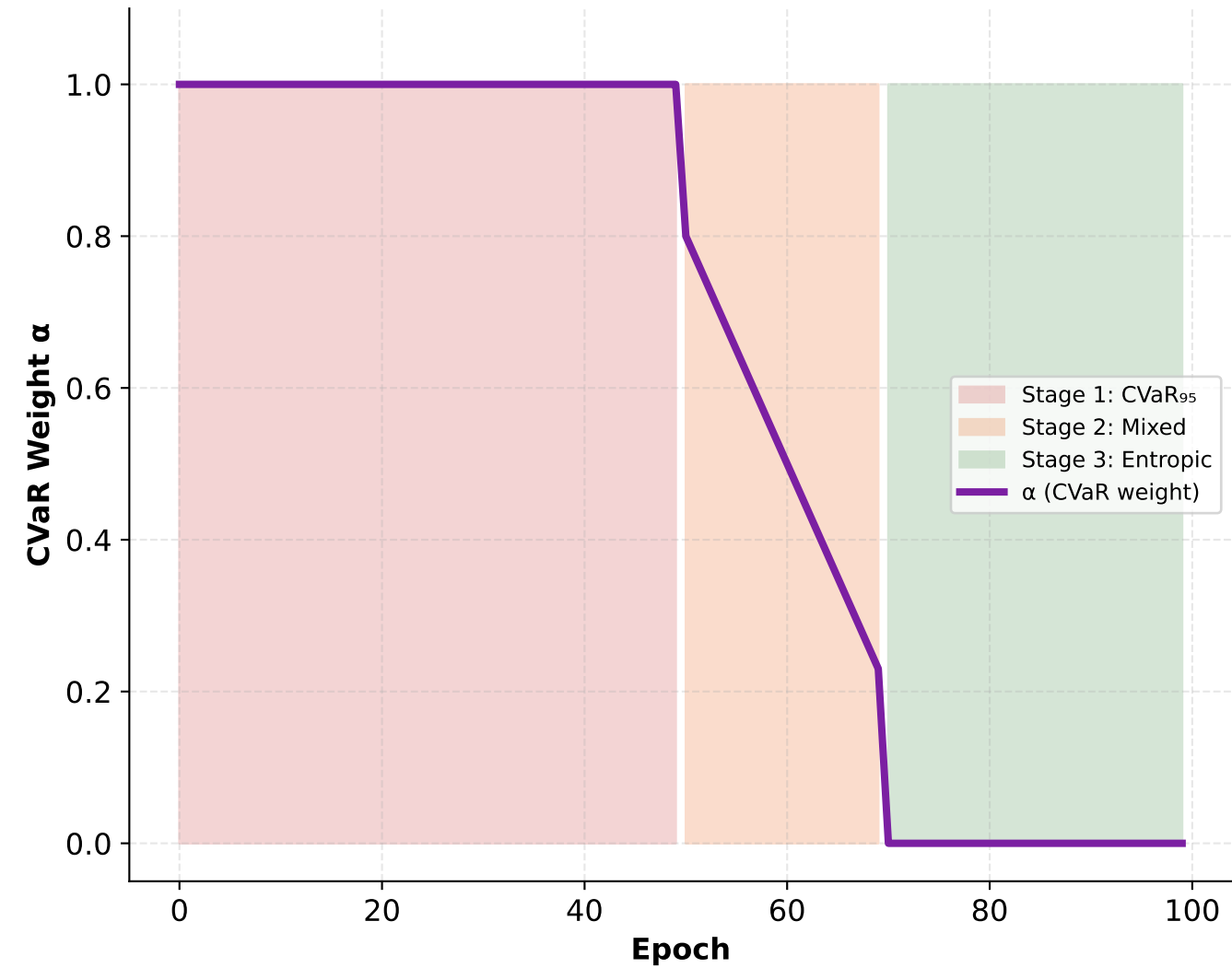
3SCH Curriculum Schedule
