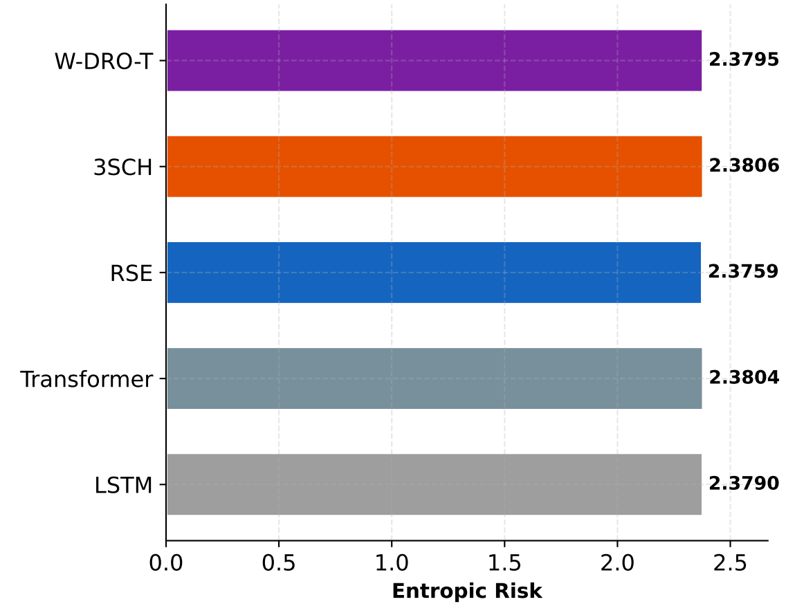
Entropic Risk (lower is better)
