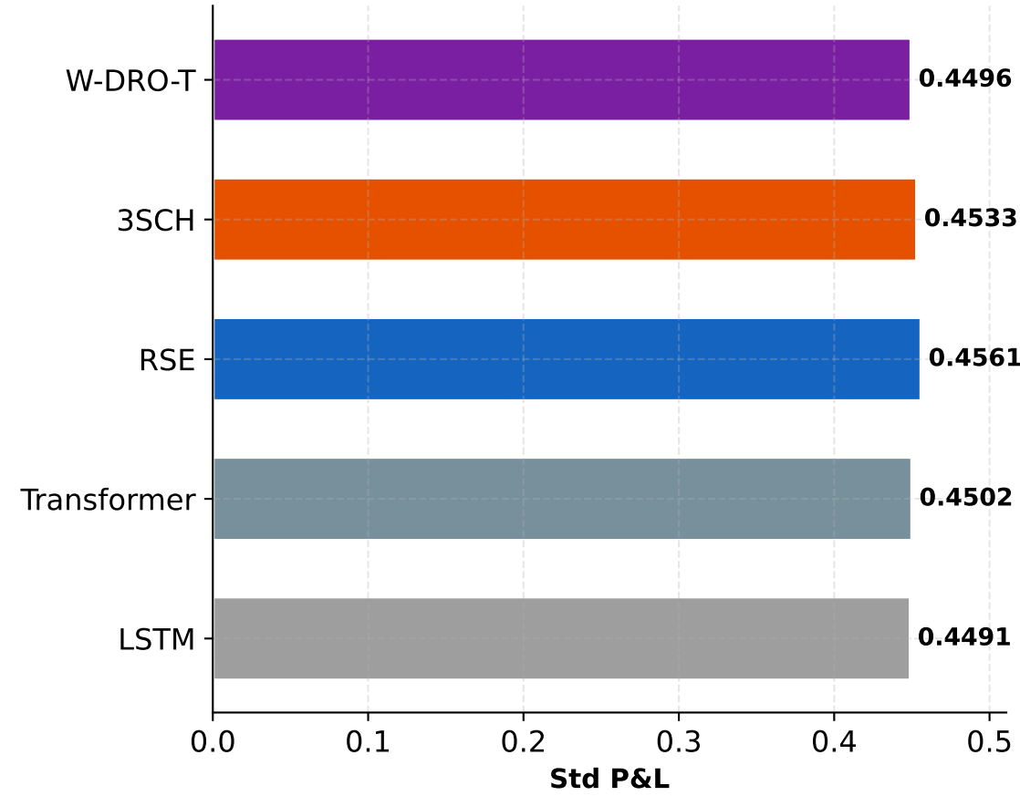
Std P&L (lower is better)
