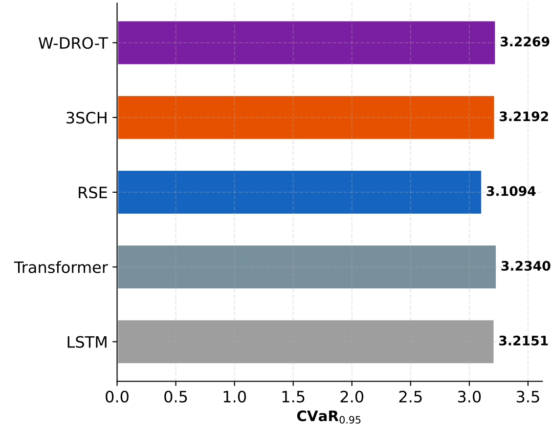
CVaR 0.95 (lower is better)
