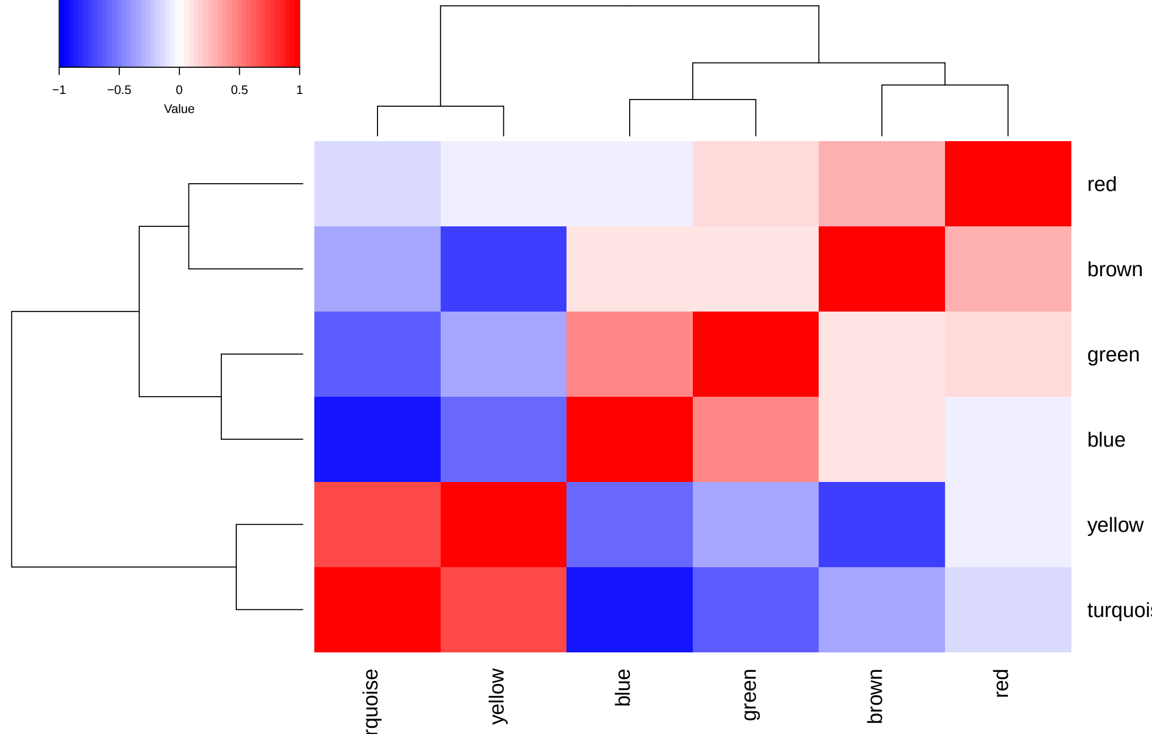
Normal Module Correlation (UNSIGNED)
