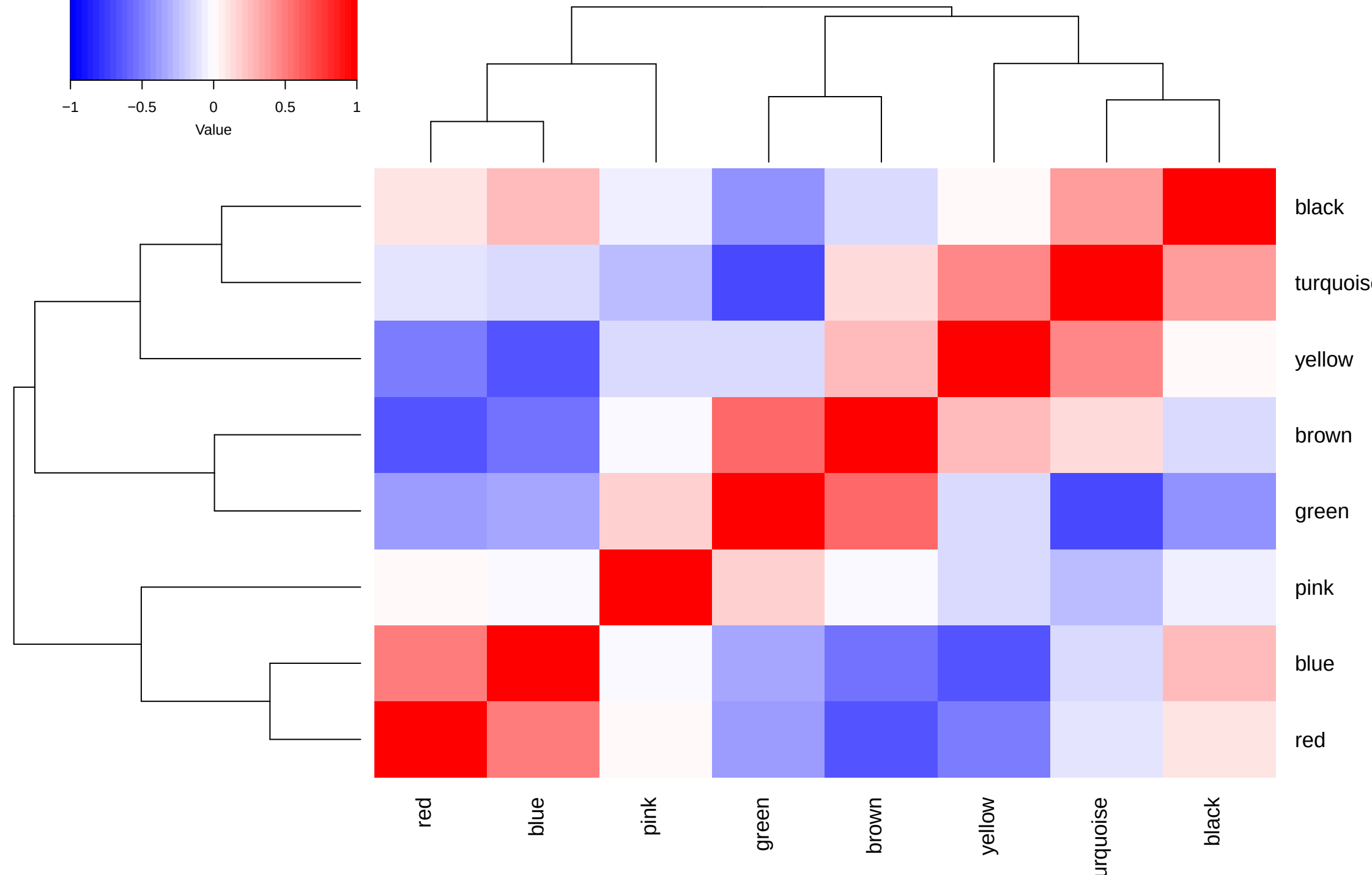
Tumor Module Correlation (UNSIGNED)
