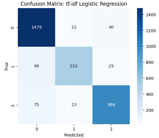
Fig. 2. TF-IDF confusion matrix.
