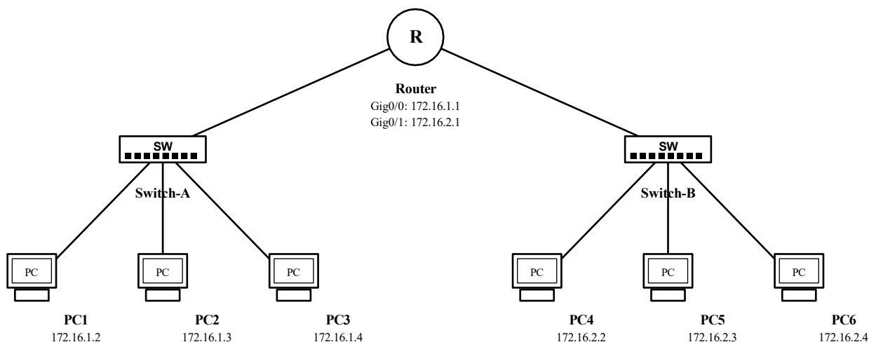
Fig 3: Lab inter-network using switches, router and Ethernet cables (Part c)
