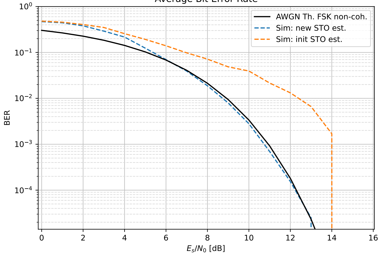
Average Bit Error Rate
