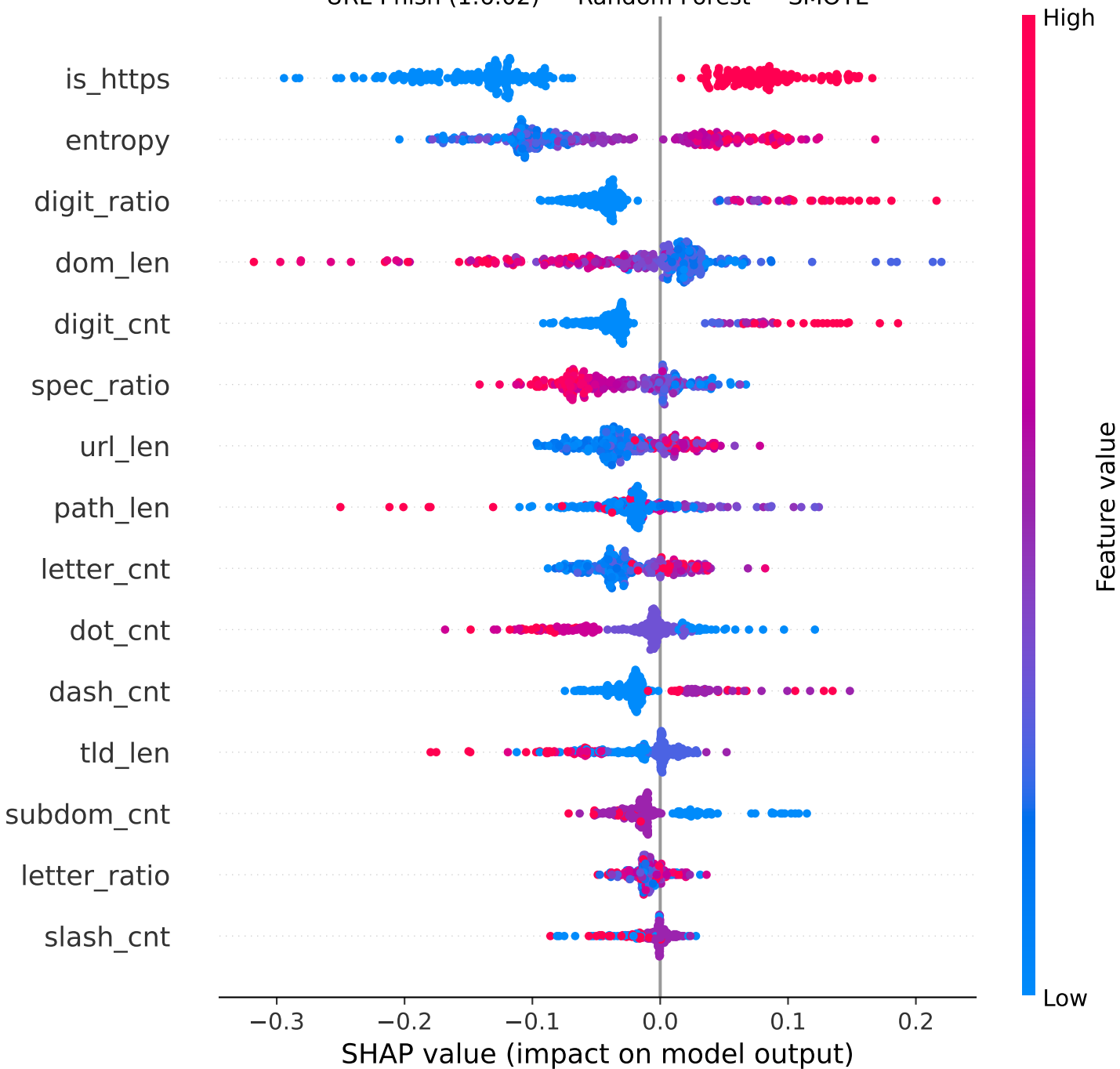
URL-Phish (1:6.02) - Random Forest - SMOTE
