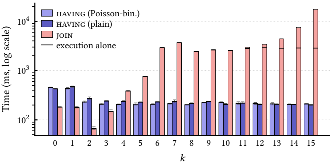
COUNT(*) \geq k (probability)
