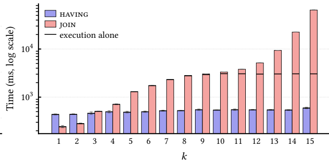
COUNT(*) \leq k (probability)
