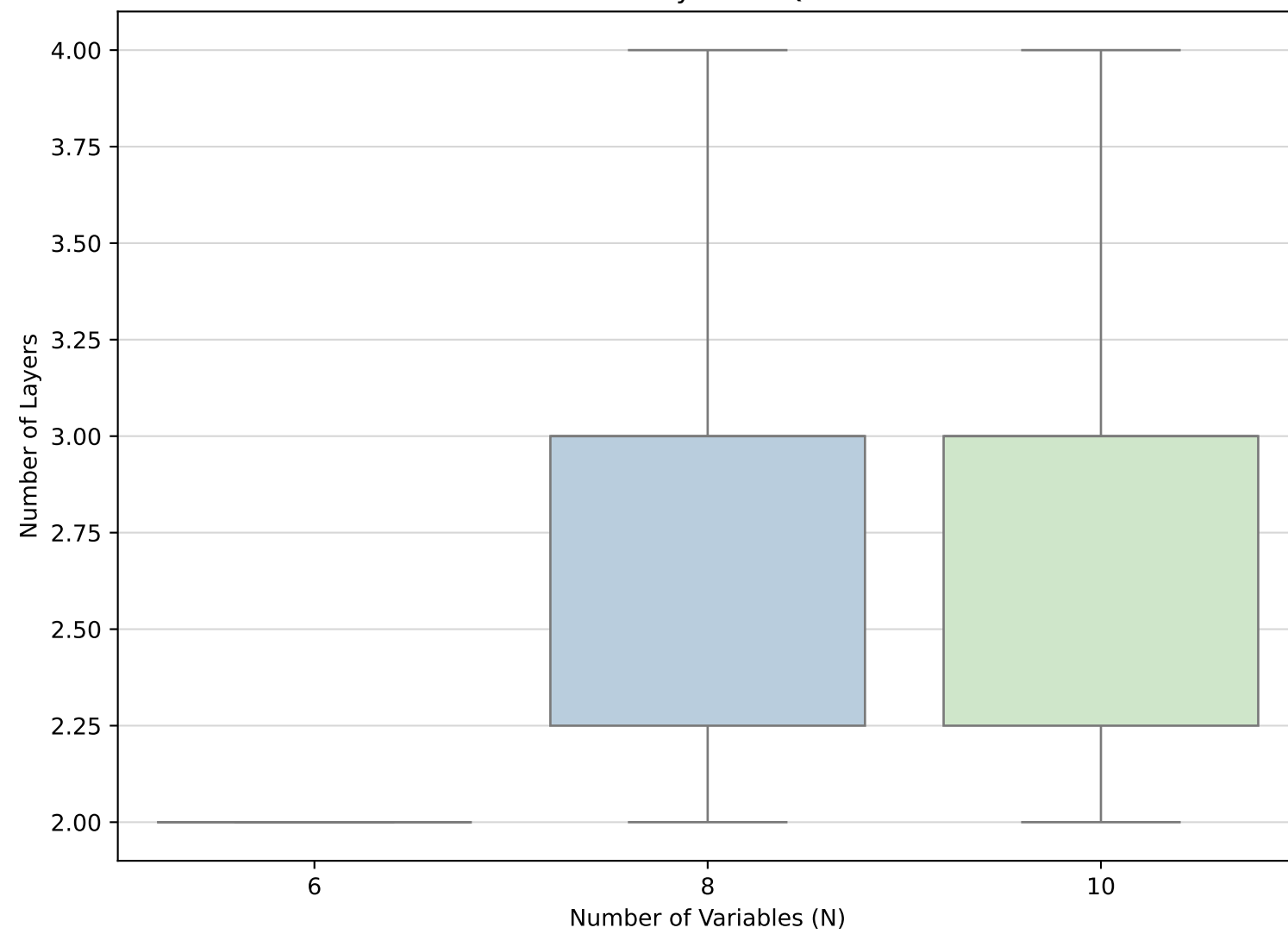
ADAPT Layers vs Qubits
