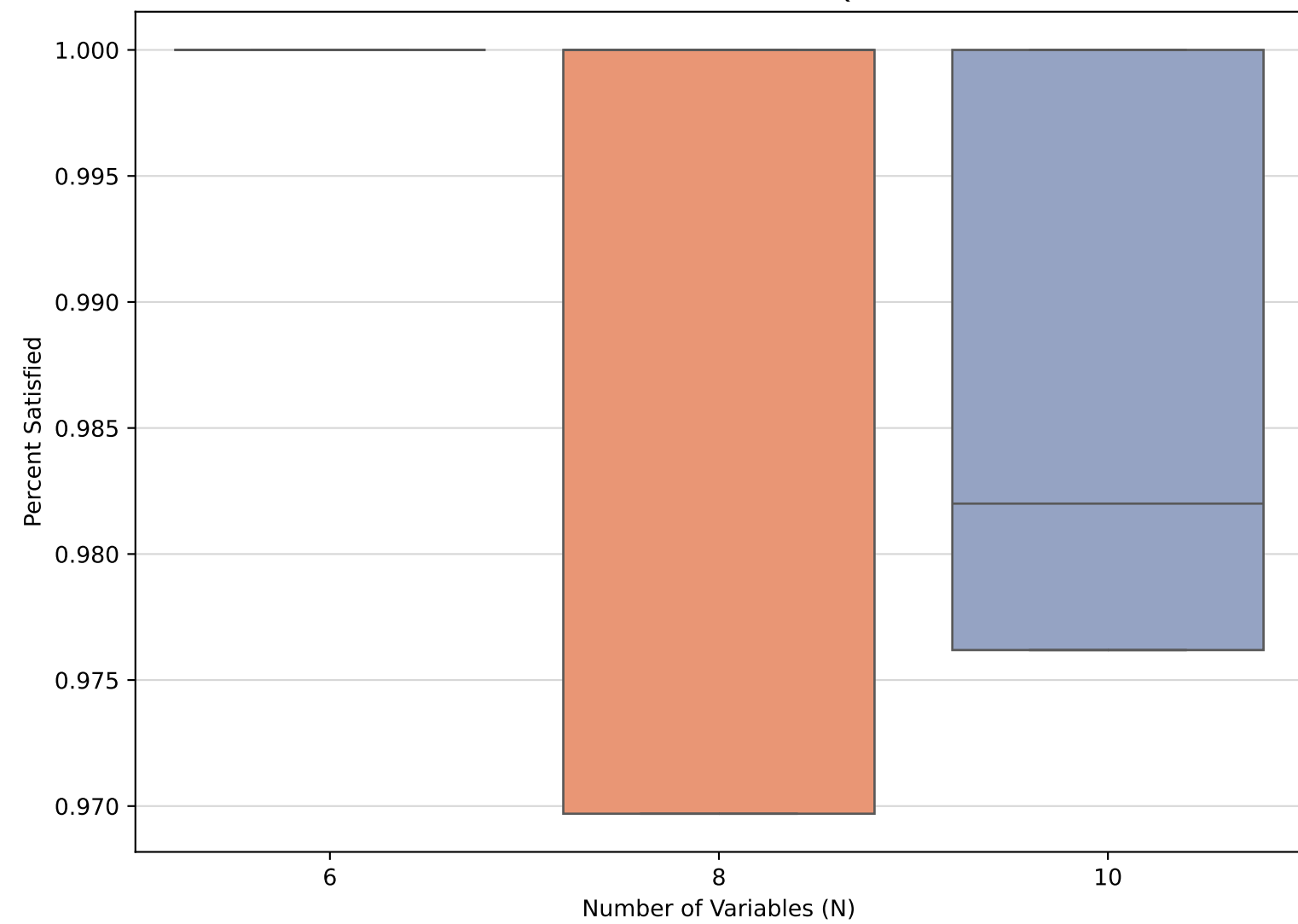
Satisfied Clauses % vs Qubits
