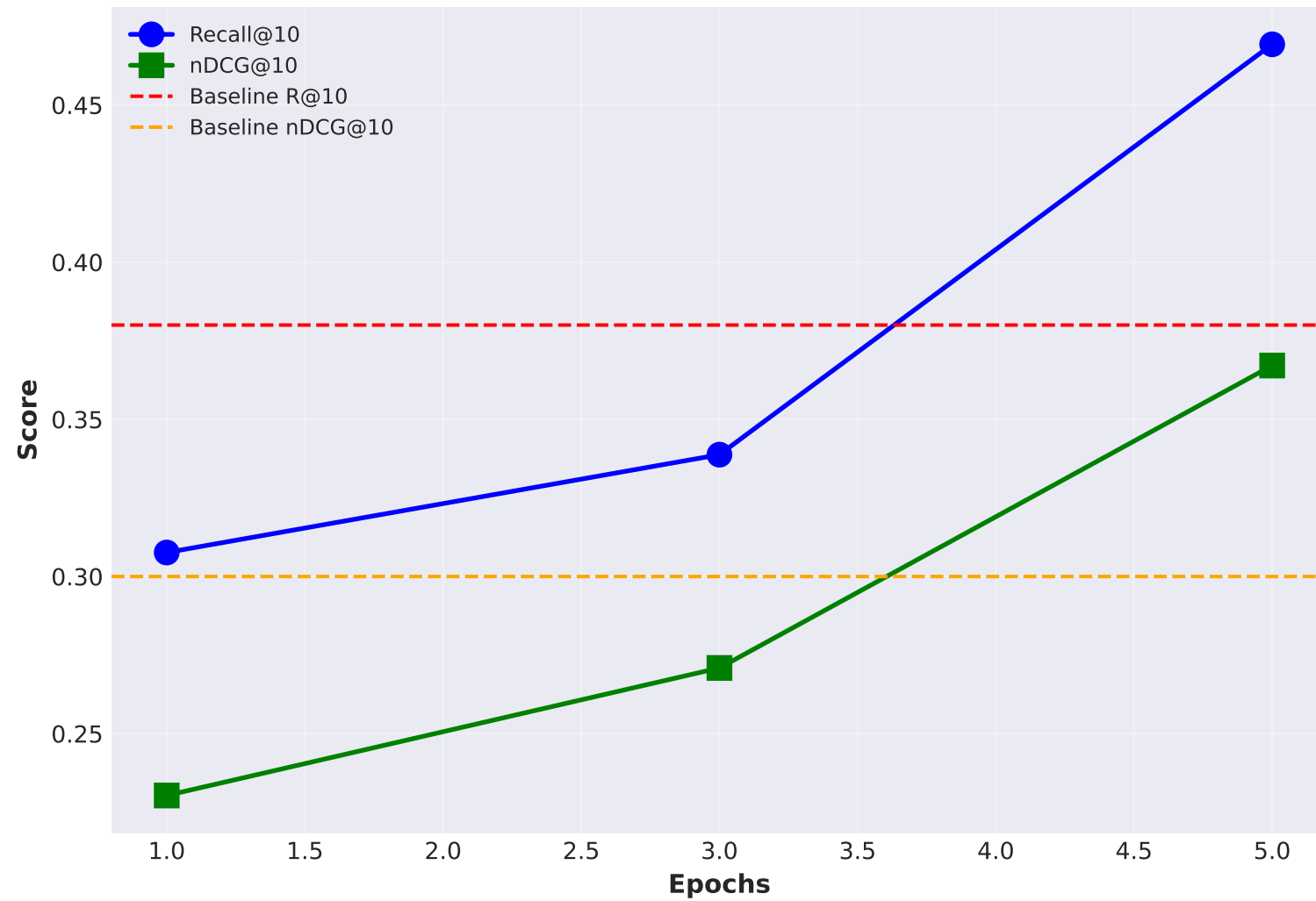
Impact of Data Augmentation
