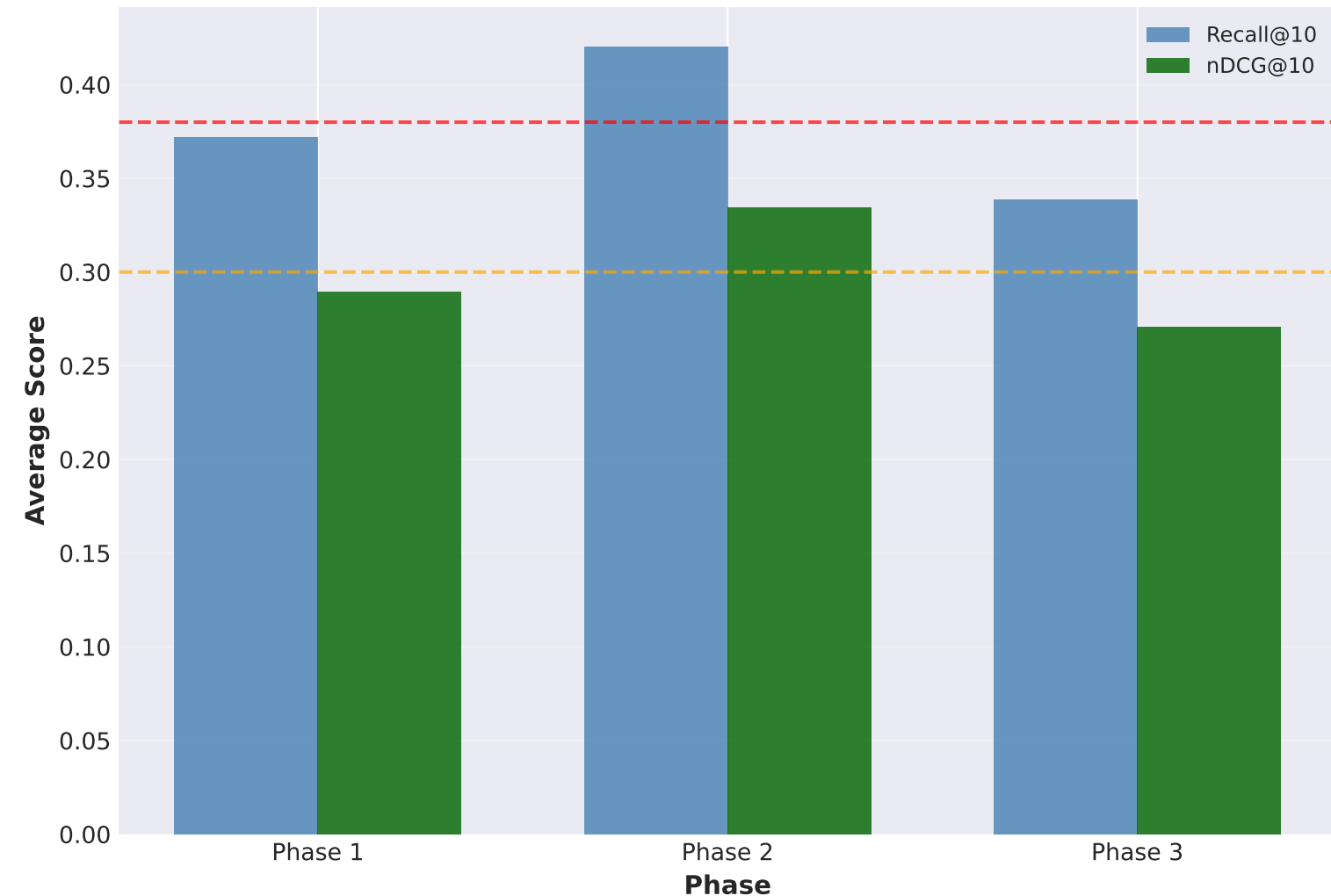
Average Performance by Phase
