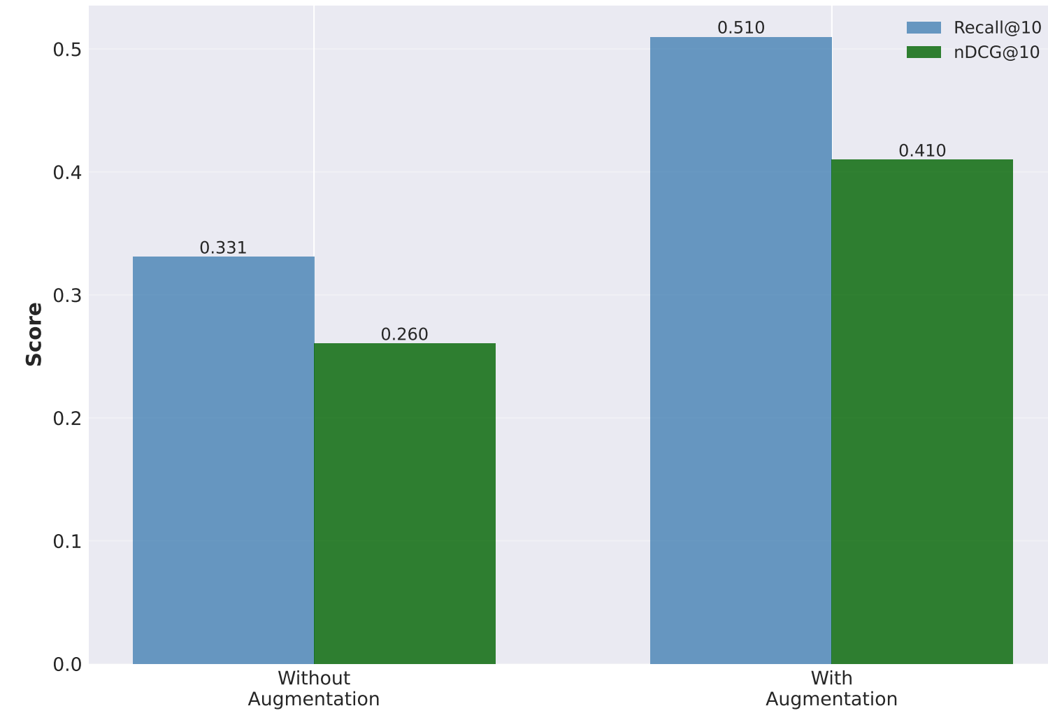
Impact of Data Augmentation
