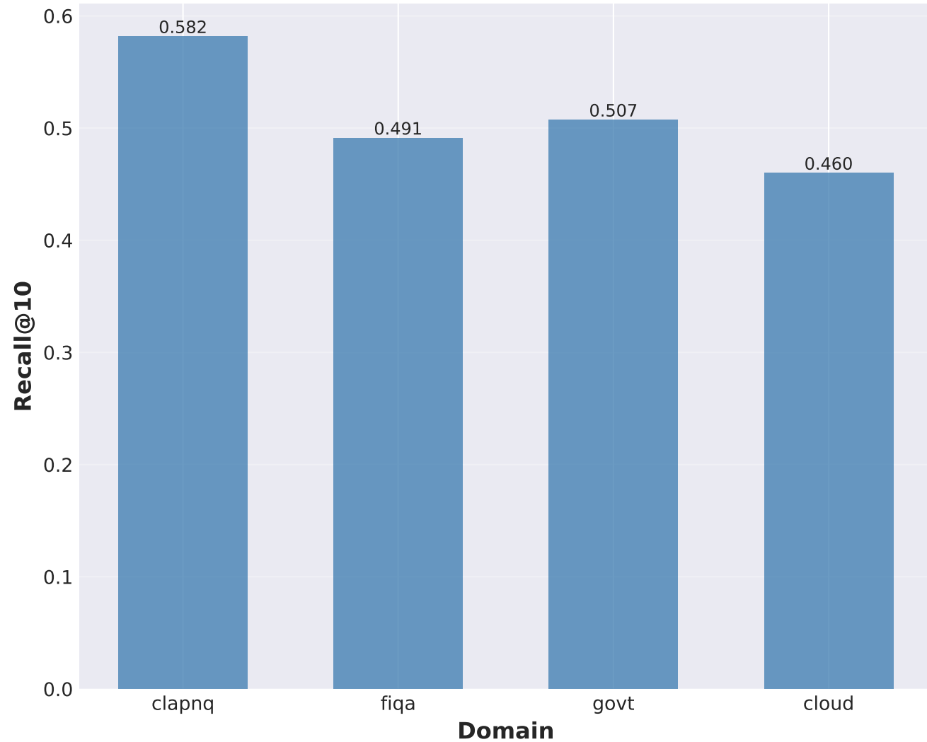
Domain-specific Recall@10 (Best Model: phase2_augmentation)
