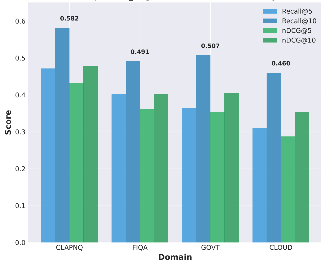
Best Model (phase2_augmentation): All Metrics by Domain
