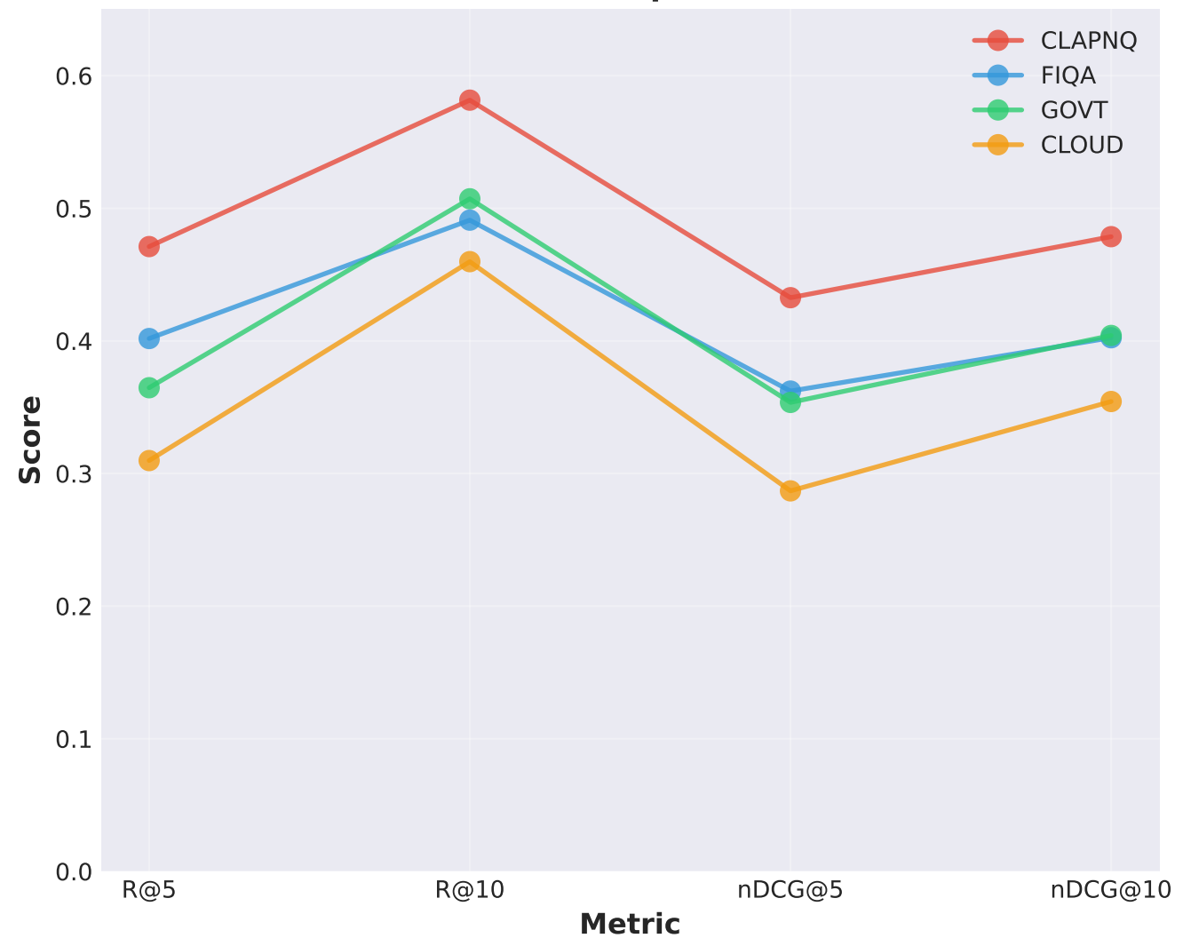
Best Model: Domain Comparison Across Metrics
