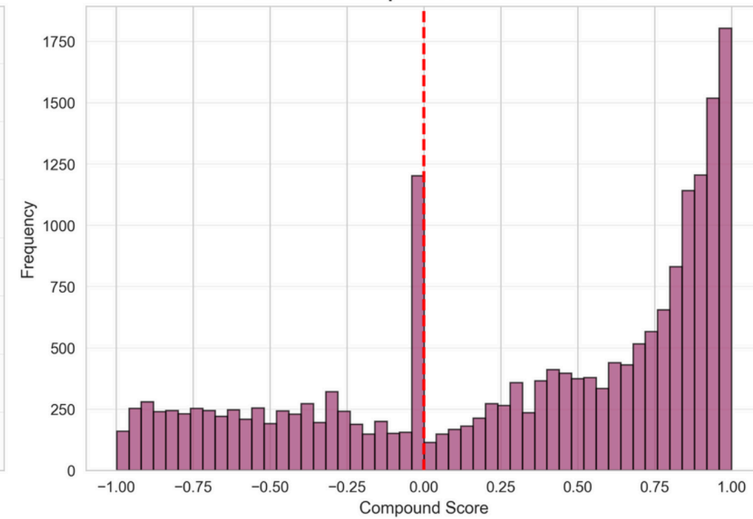
Comments: Compound Score Distribution
