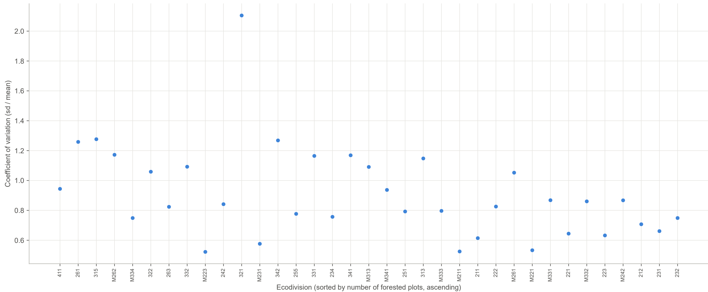
Coefficient of variation of carbon density by ecodivision, sorted by sample size
