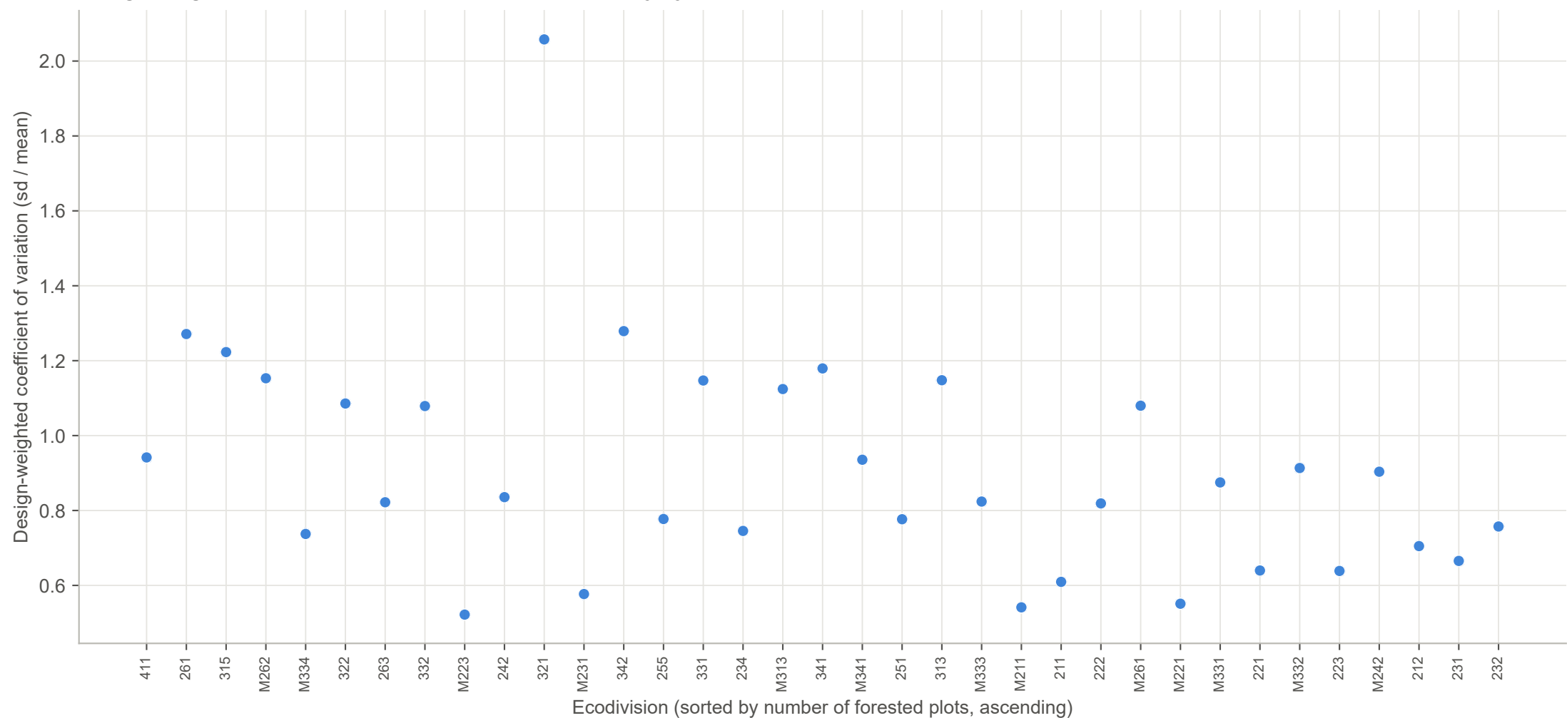
Design-weighted coefficient of variation of carbon density by ecodivision
