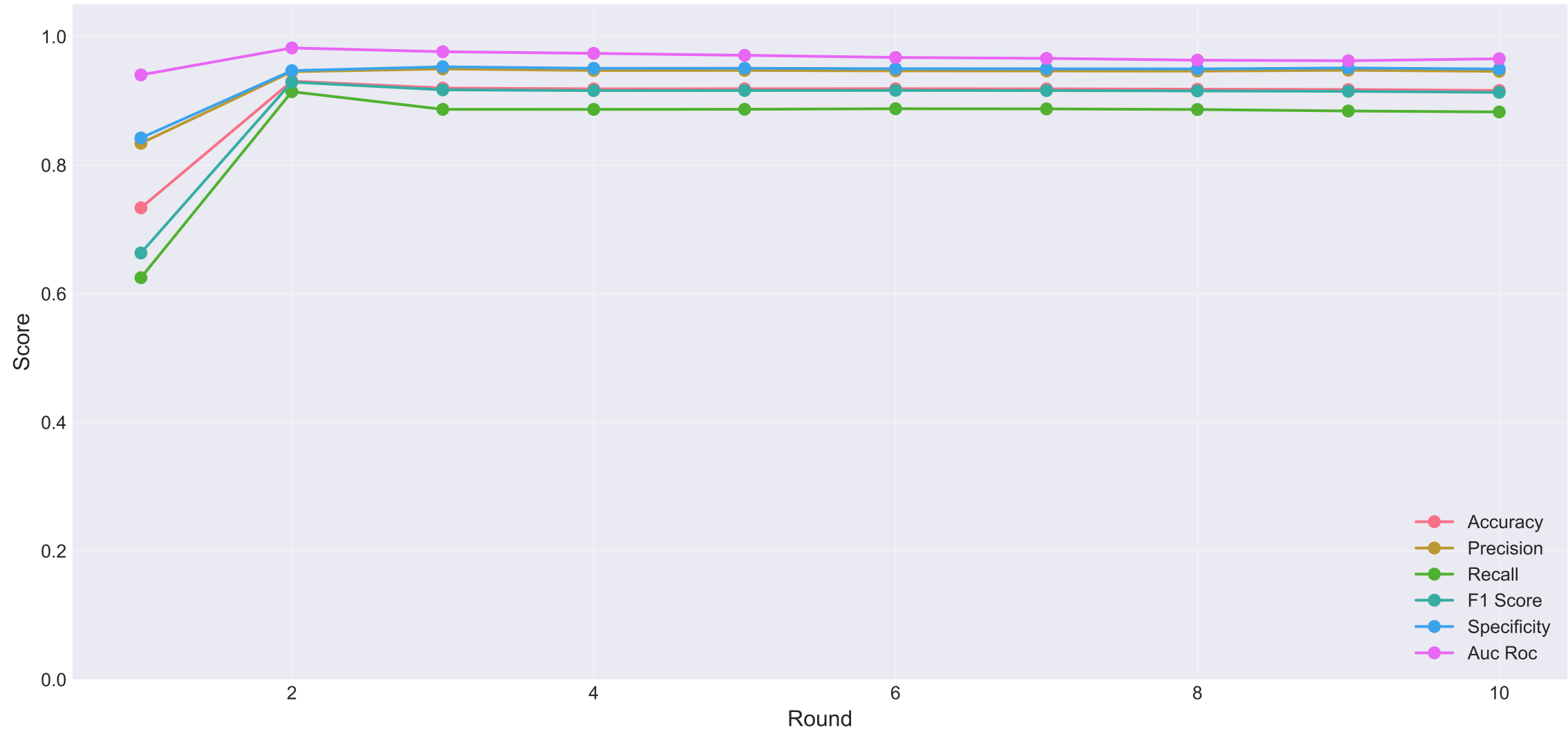
Model Performance Convergence Over Federated Learning Rounds
