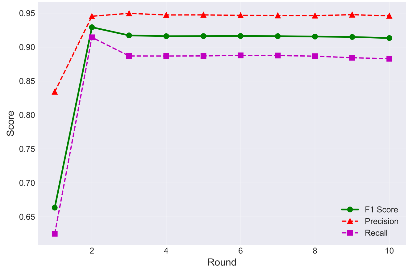
Learning Curve: Detection Metrics
