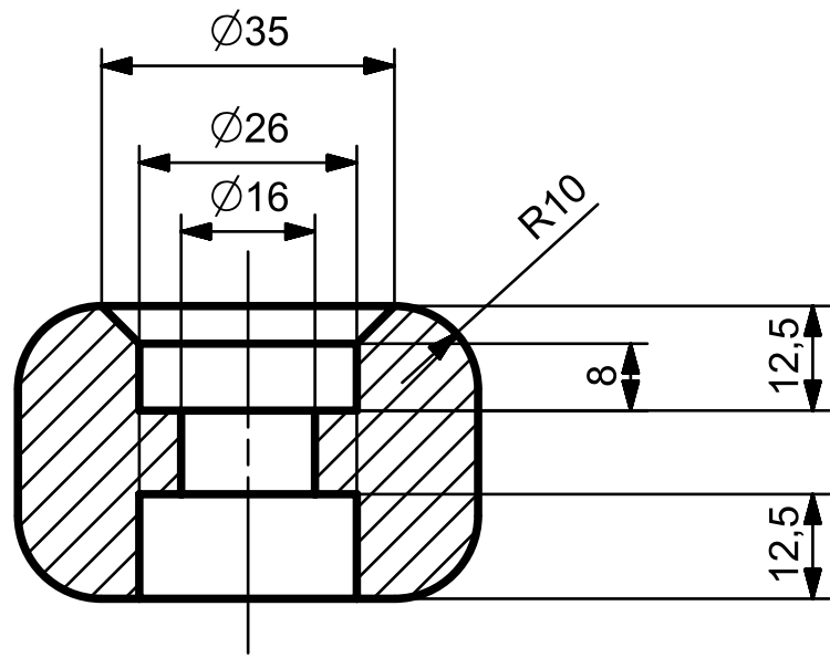
SECTION N-N
