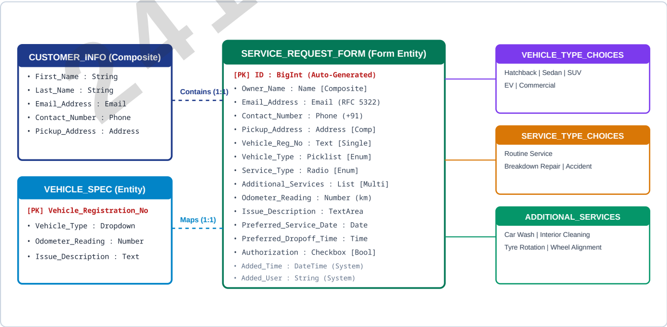
Figure 1: Entity-Relationship (ER) Schema Diagram for Vehicle Service Request Form in Zoho Creator
