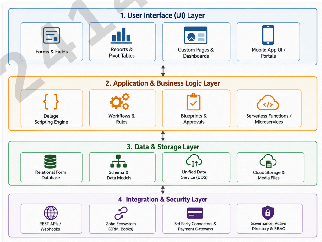
Figure 1: Zoho Creator Account & Console Architecture Overview
