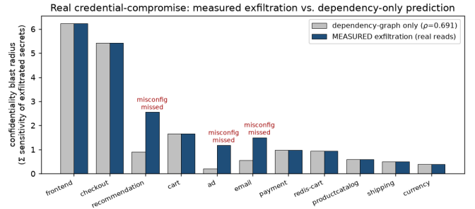
Fig. 6. Real credential-compromise on the live cluster: measured secret exfiltration vs. a dependency-only prediction. The dependency-only view misses the three planted over-privilege misconfigurations; the RBAC-aware confidentiality score reproduces the exfiltrated set.
