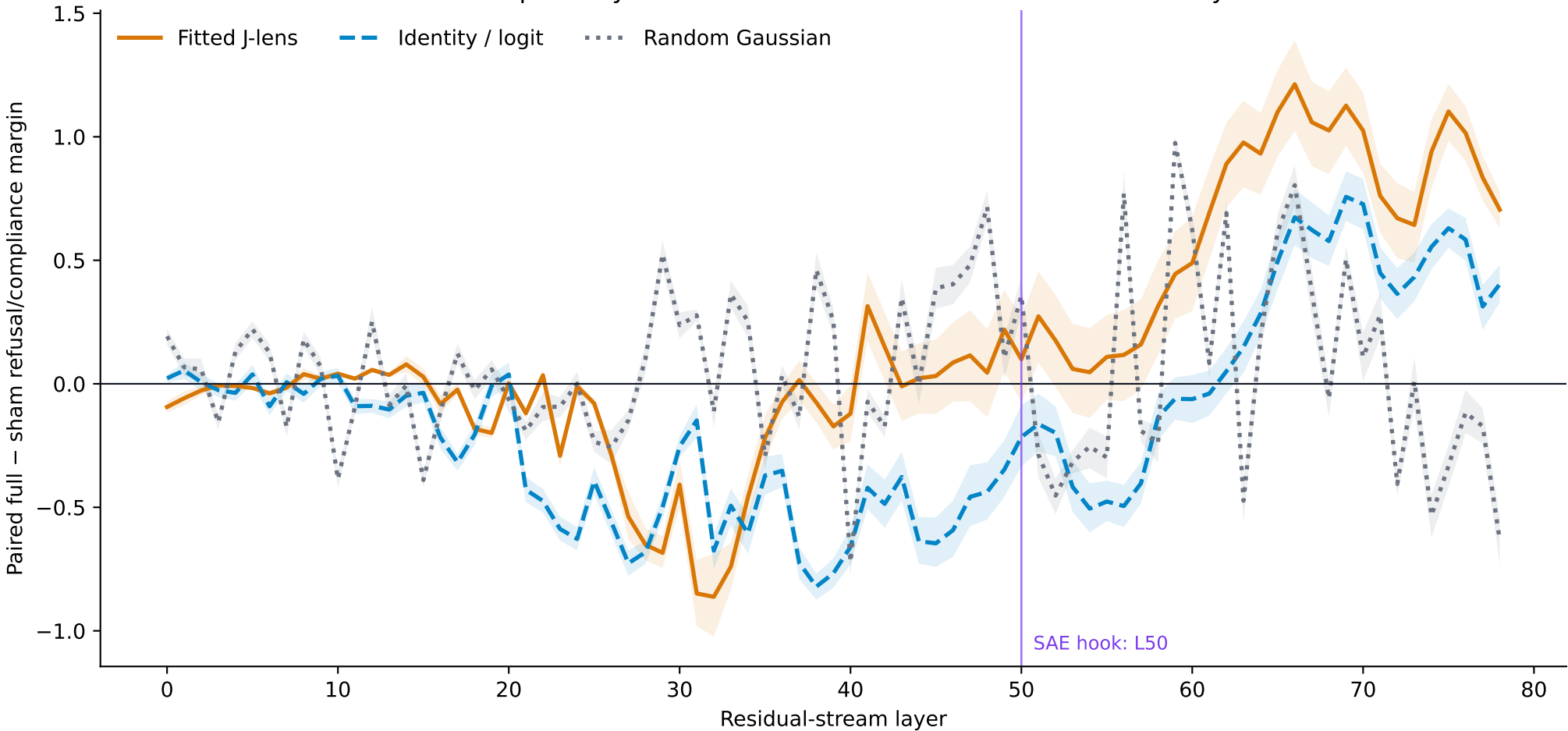
Descriptive layerwise readout at the turn-2 assistant boundary
