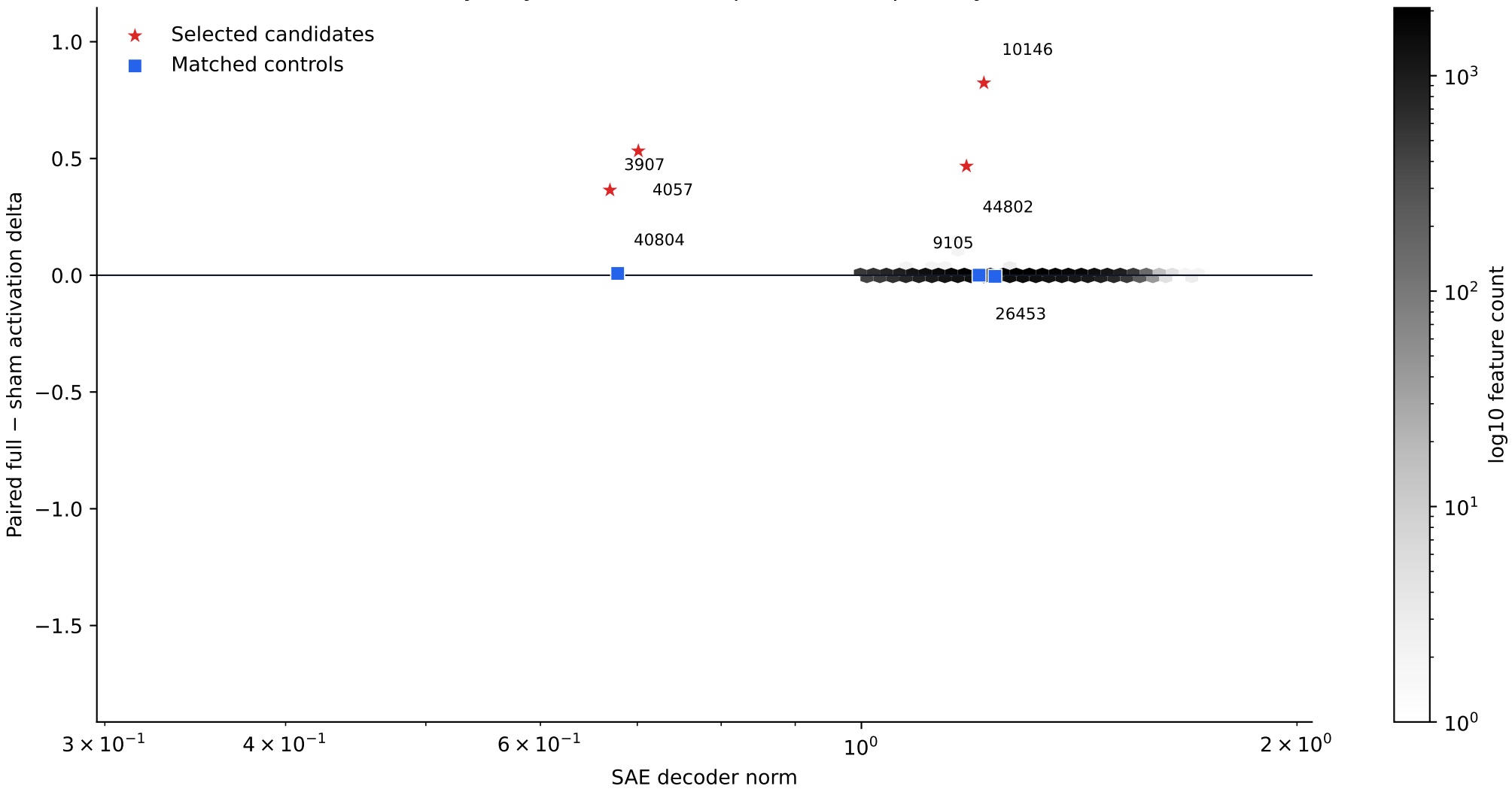
Discovery-only SAE feature map at residual-post layer 50
