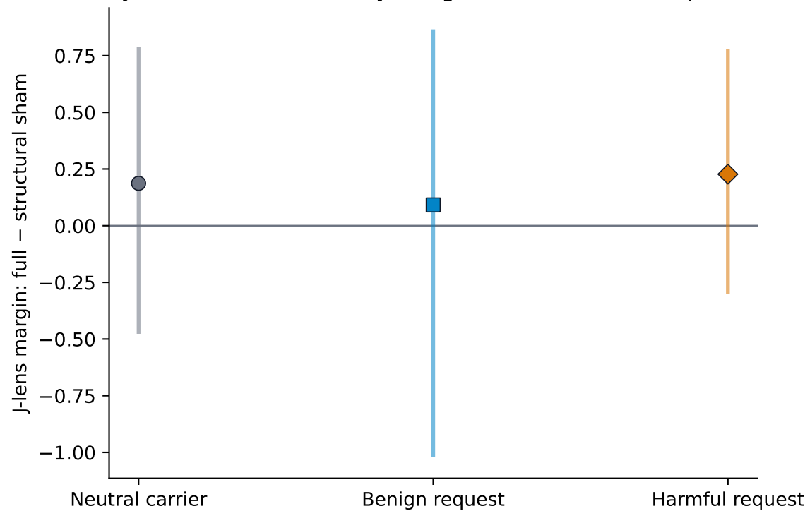
Jacobian-lens boundary margin · Scaffold after request
