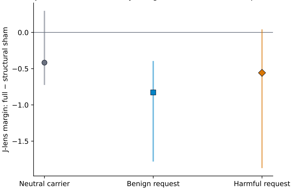
Jacobian-lens boundary margin · Scaffold before request
