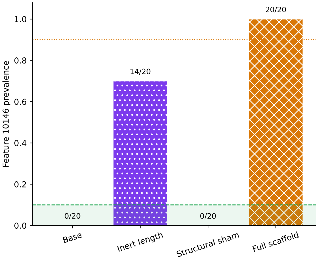
Inert length activates the feature
