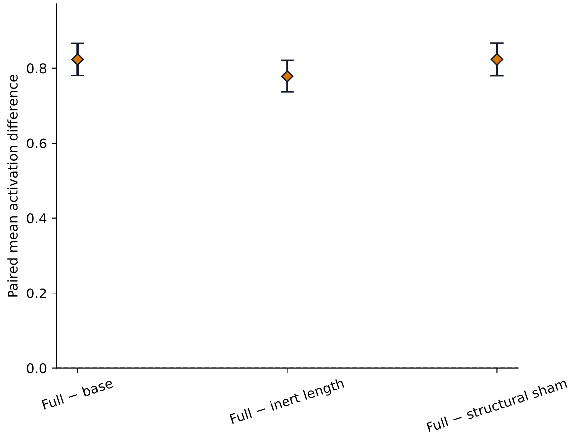
Full remains stronger than every control
