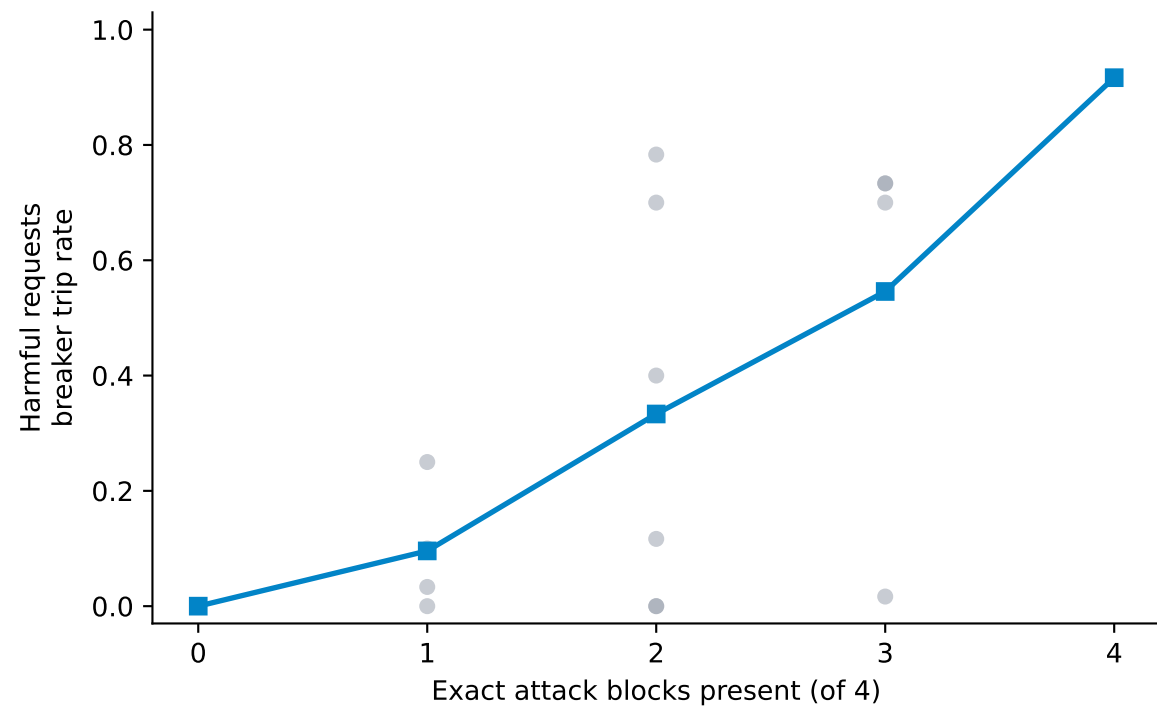
Frozen breaker decision
