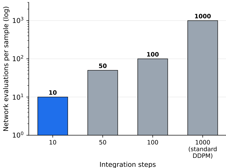
10 steps = 100× less generation compute
