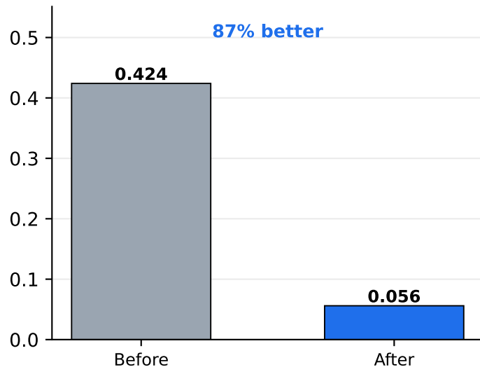
Discrete-column fix U2R distribution error
