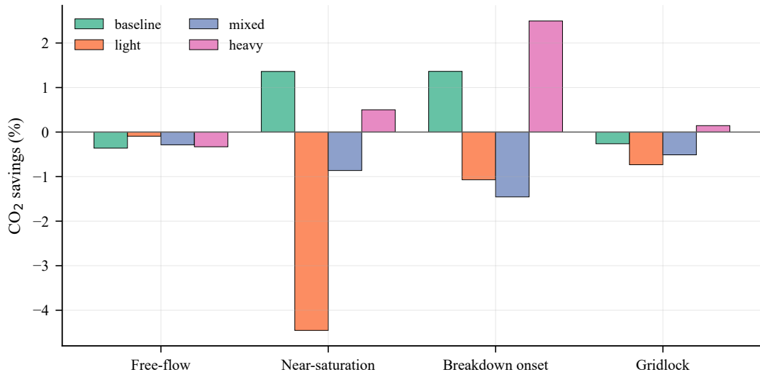
CO 2 savings by fleet composition and regime
