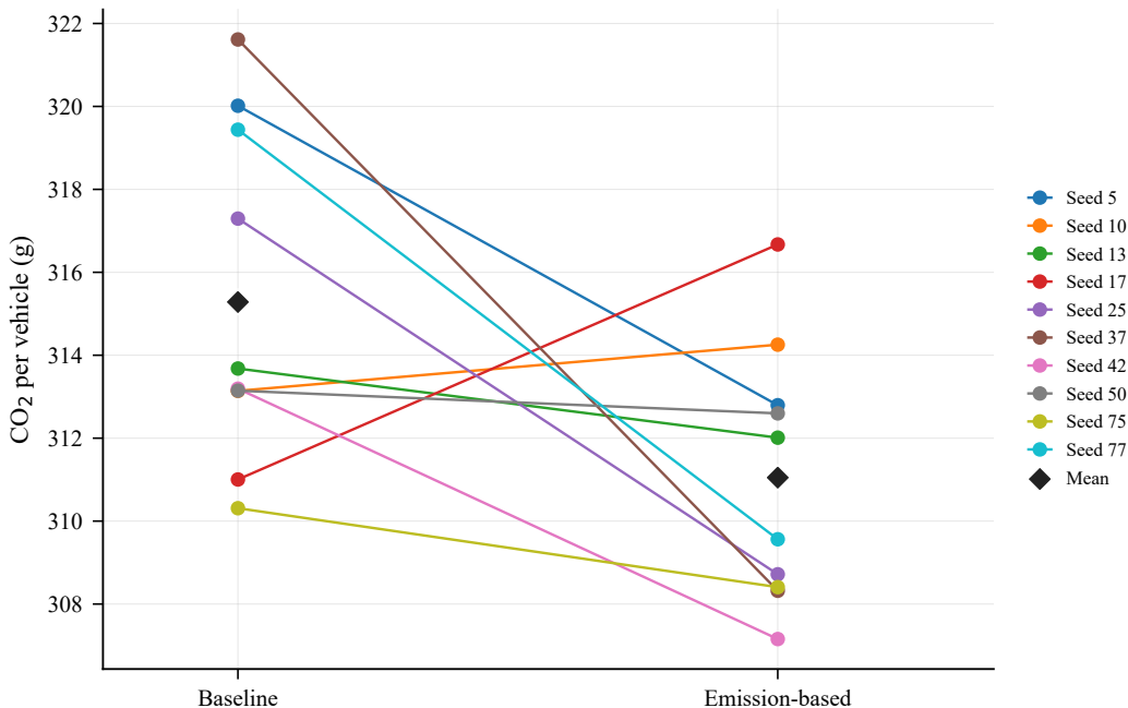
V2900 — paired-seed CO 2 /vehicle (n = 10 seeds)
