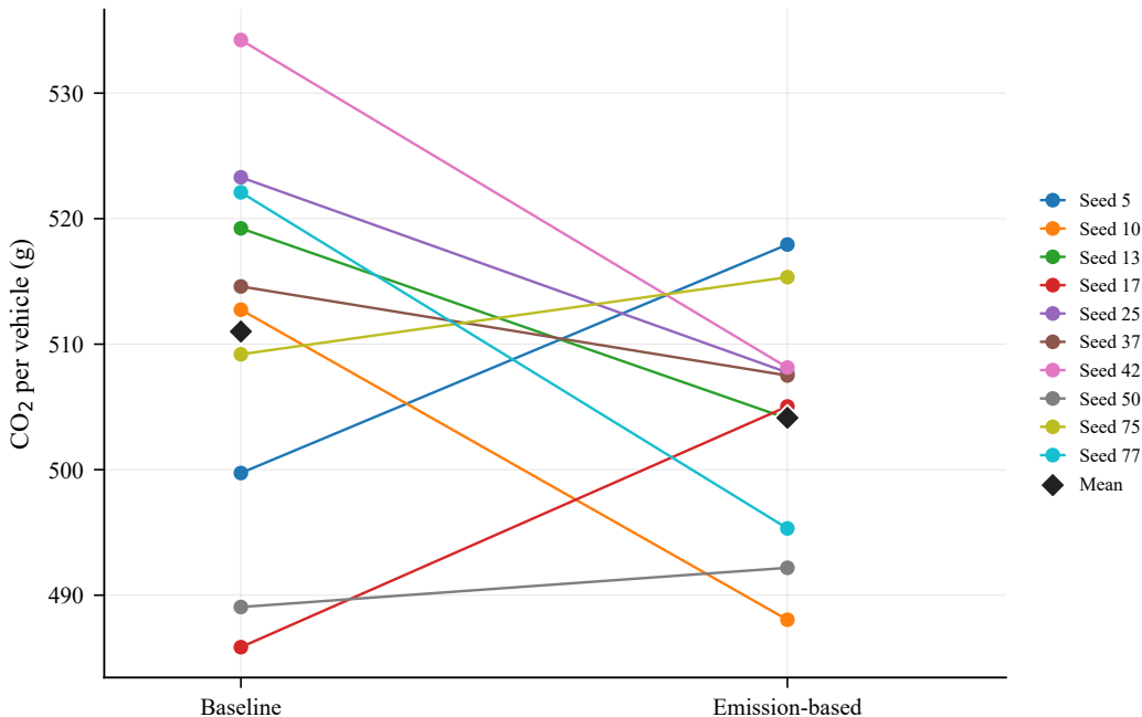
V3300 — paired-seed CO 2 /vehicle (n = 10 seeds)
