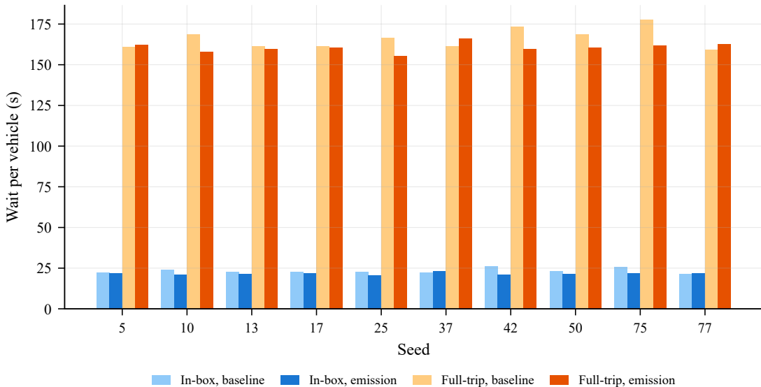
V5000 — in-box vs full-trip wait, by seed
