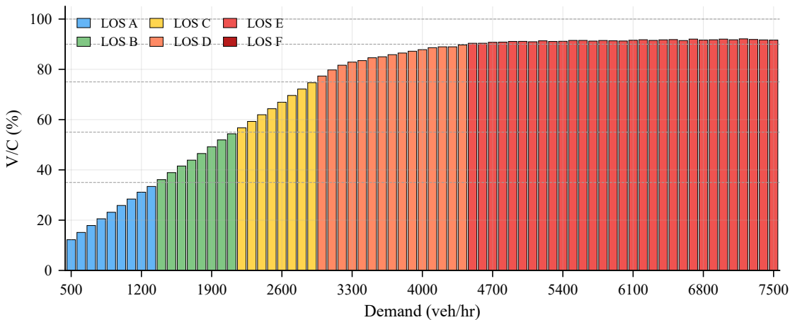
(c) Per-cycle V/C (%) with LOS proxy bands — critical V = 7400
