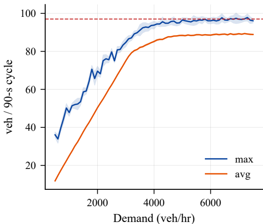
(a) Discharge/cycle — cap = 97
