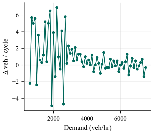
(b) \Delta max per +100 veh/hr
