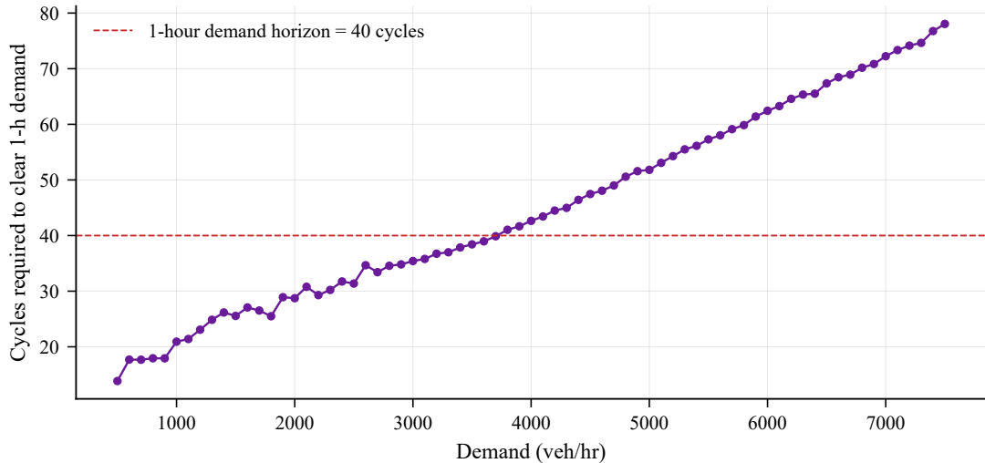
Cycles required to clear 1-hour demand at peak discharge
