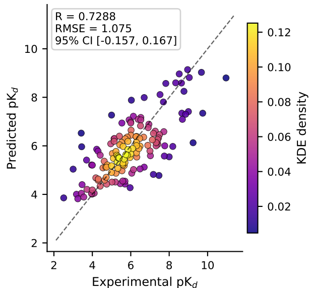
(b) Predicted vs. Experimental pK_d
