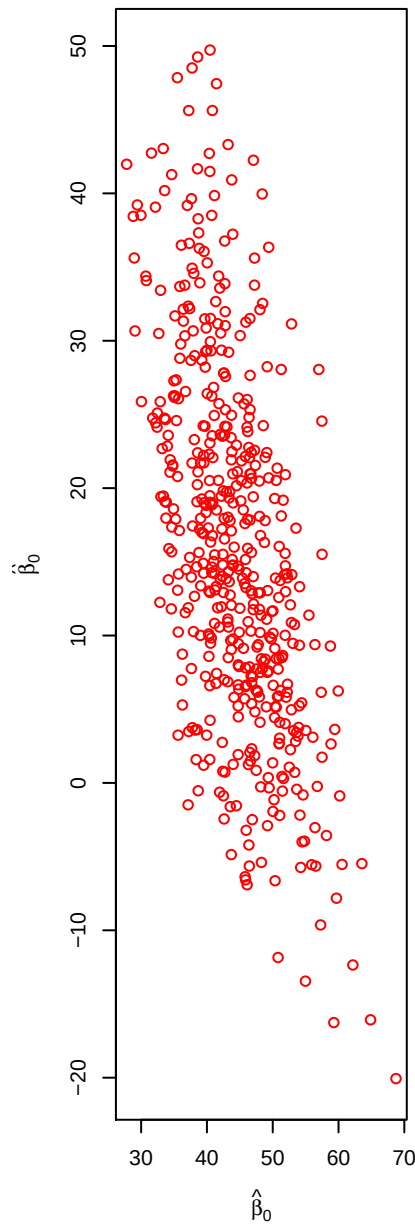
Joint Distribution of \hat{\beta}_0
