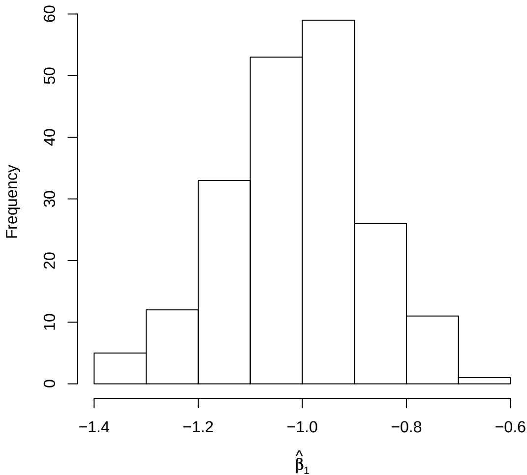
Sampling distribution of \hat{\beta}_1
