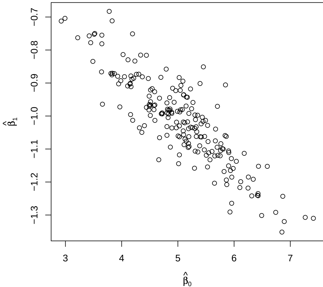
Joint sampling distribution of \hat{\beta}_0 and \hat{\beta}_1
