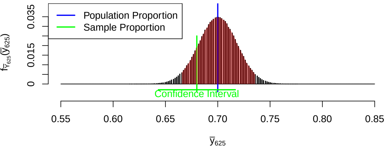
Sampling Distribution of \bar{Y}_{625}
