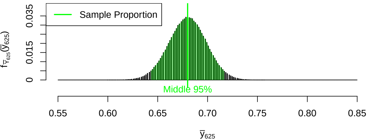
Estimated Sampling Distribution of \bar{Y}_{625}
